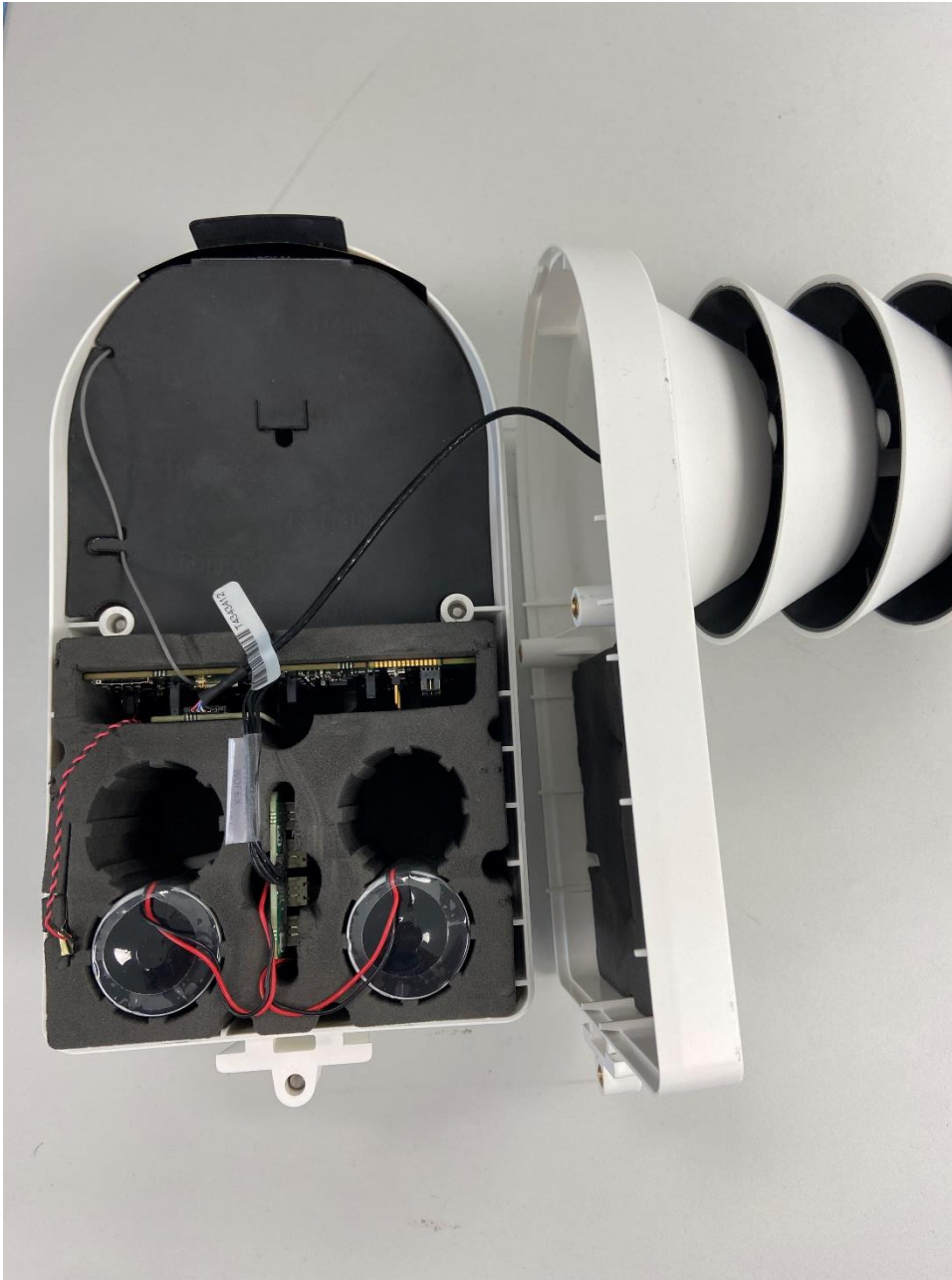
Photo 6. FMP102 opened, top view
