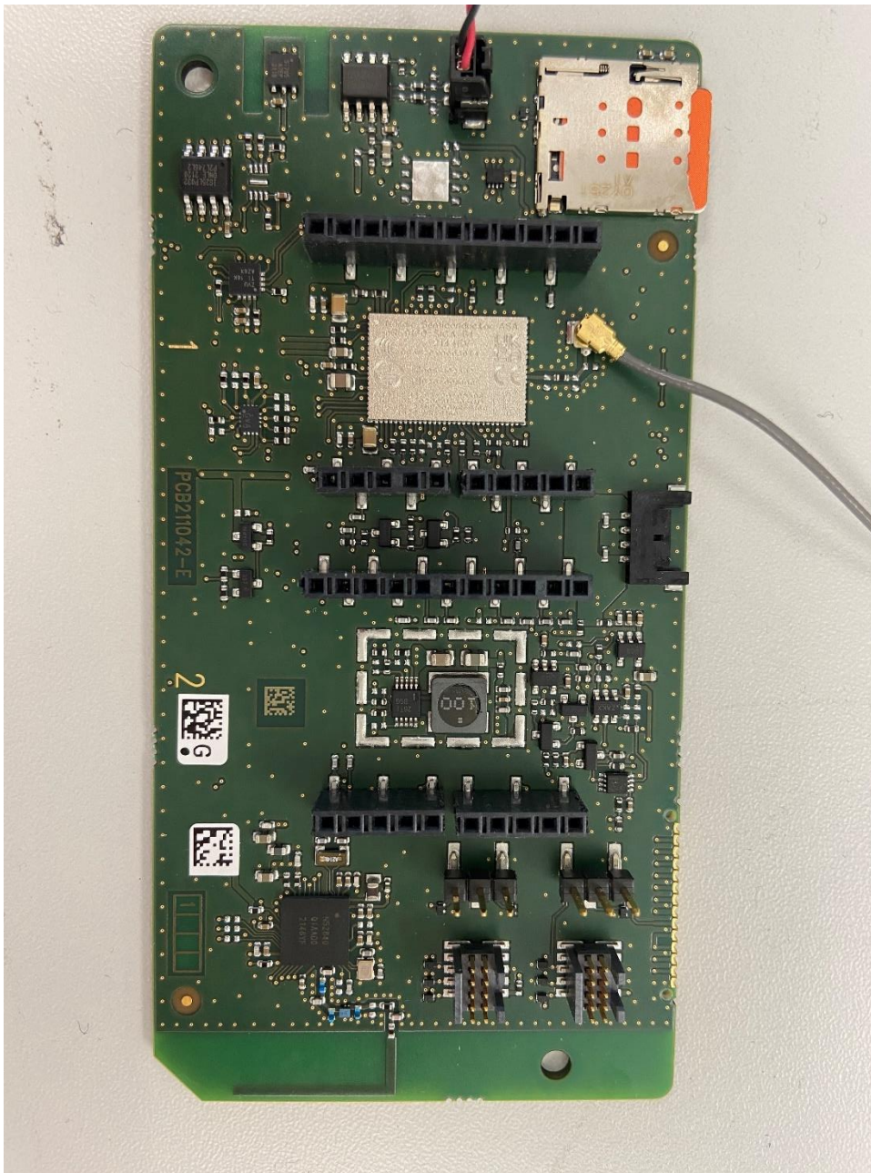
Photo 11. IOTMAIN CB, front view
