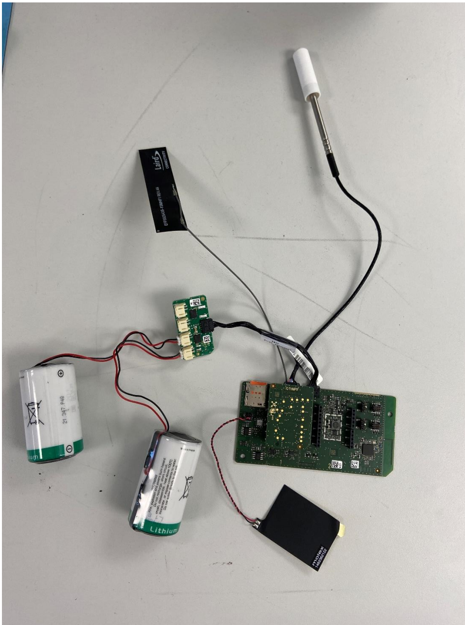
Photo 8. FMP102 Electronics
