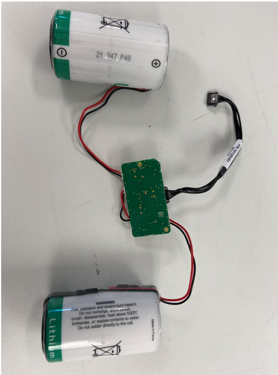
Photo 17. IOTPWR and batteries, back view
