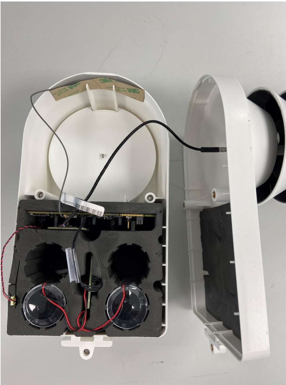
Photo 7. FMP102 opened, plastic shield removed
