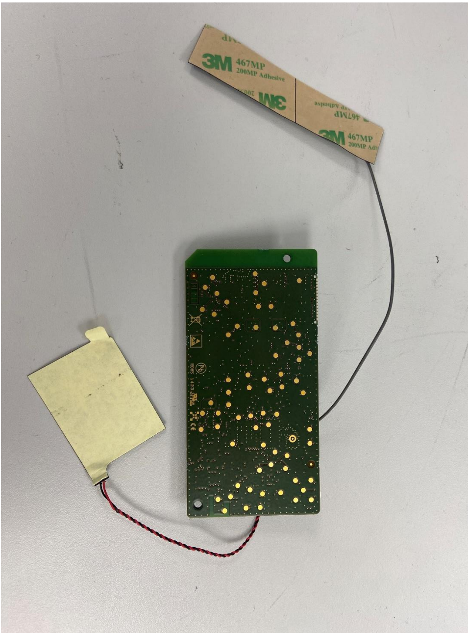
Photo 10. IOTMAINCB and Antennas, Back View
