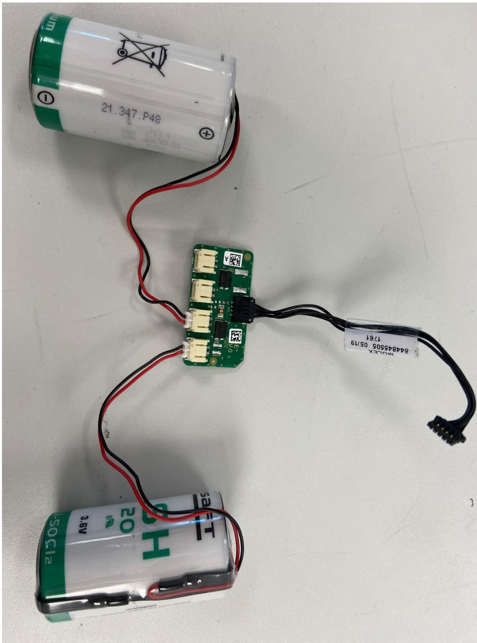
Photo 16. IOTPWR and batteries, front view
