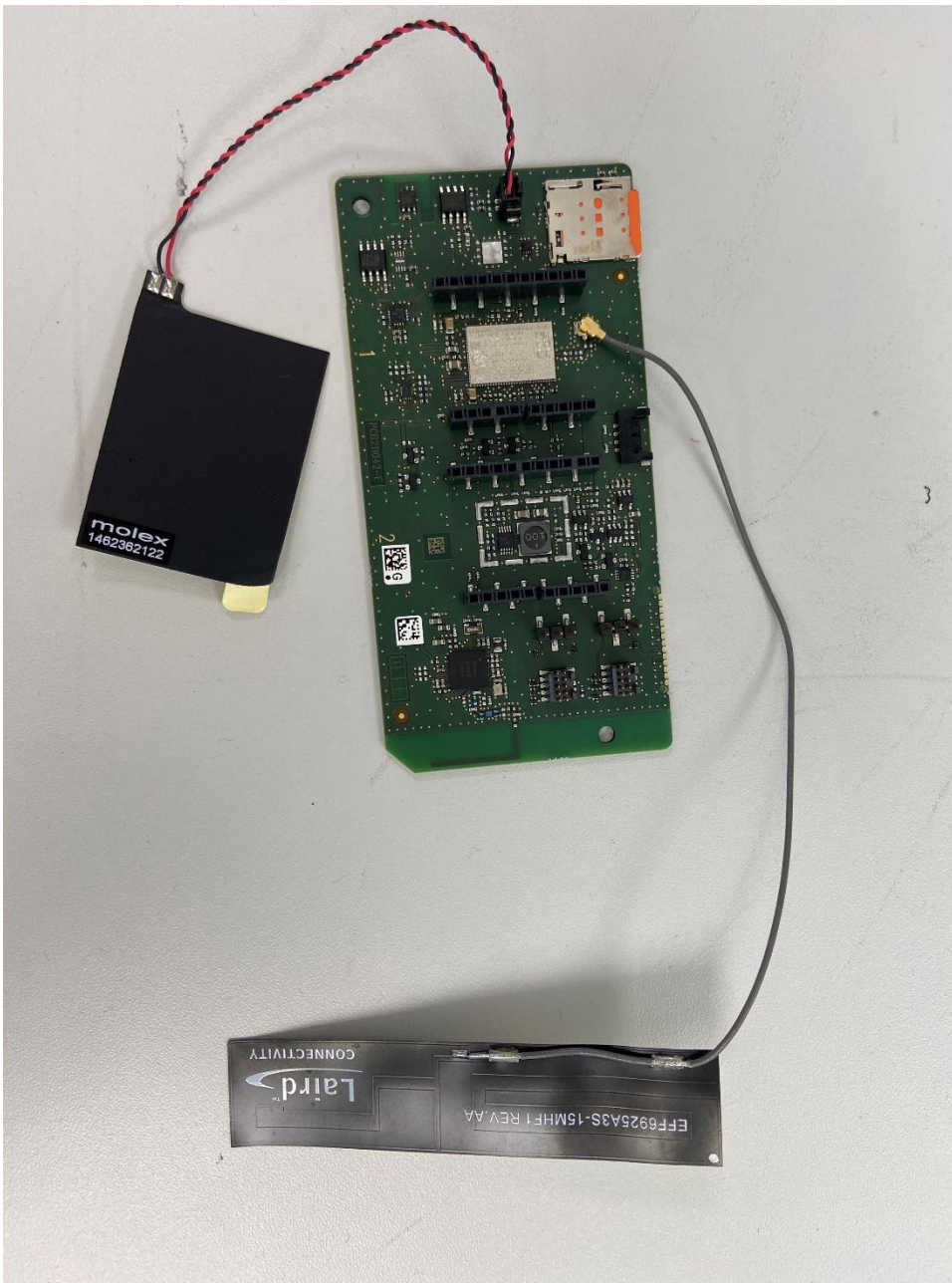
Photo 9. IOTMAINCB and Antennas, Front View
