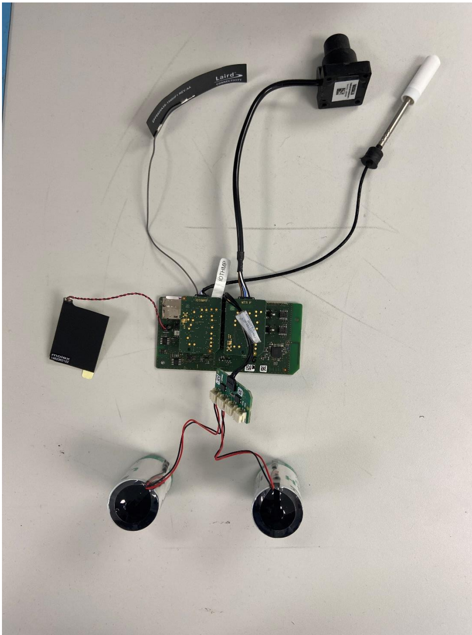
Photo 8. FMP103 Electronics
