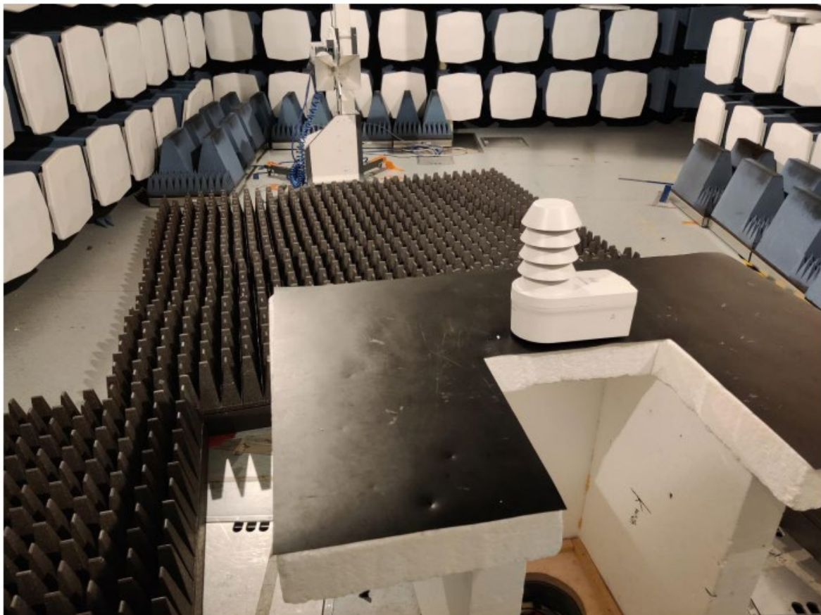
Picture 6 Radiated emission, 1– 12,75 GHz, common setup
