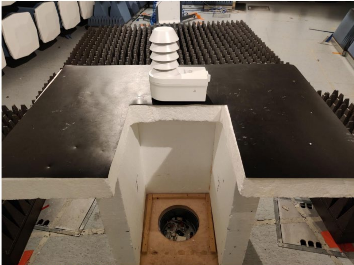
Picture 7 Radiated emission, EUT test setup
