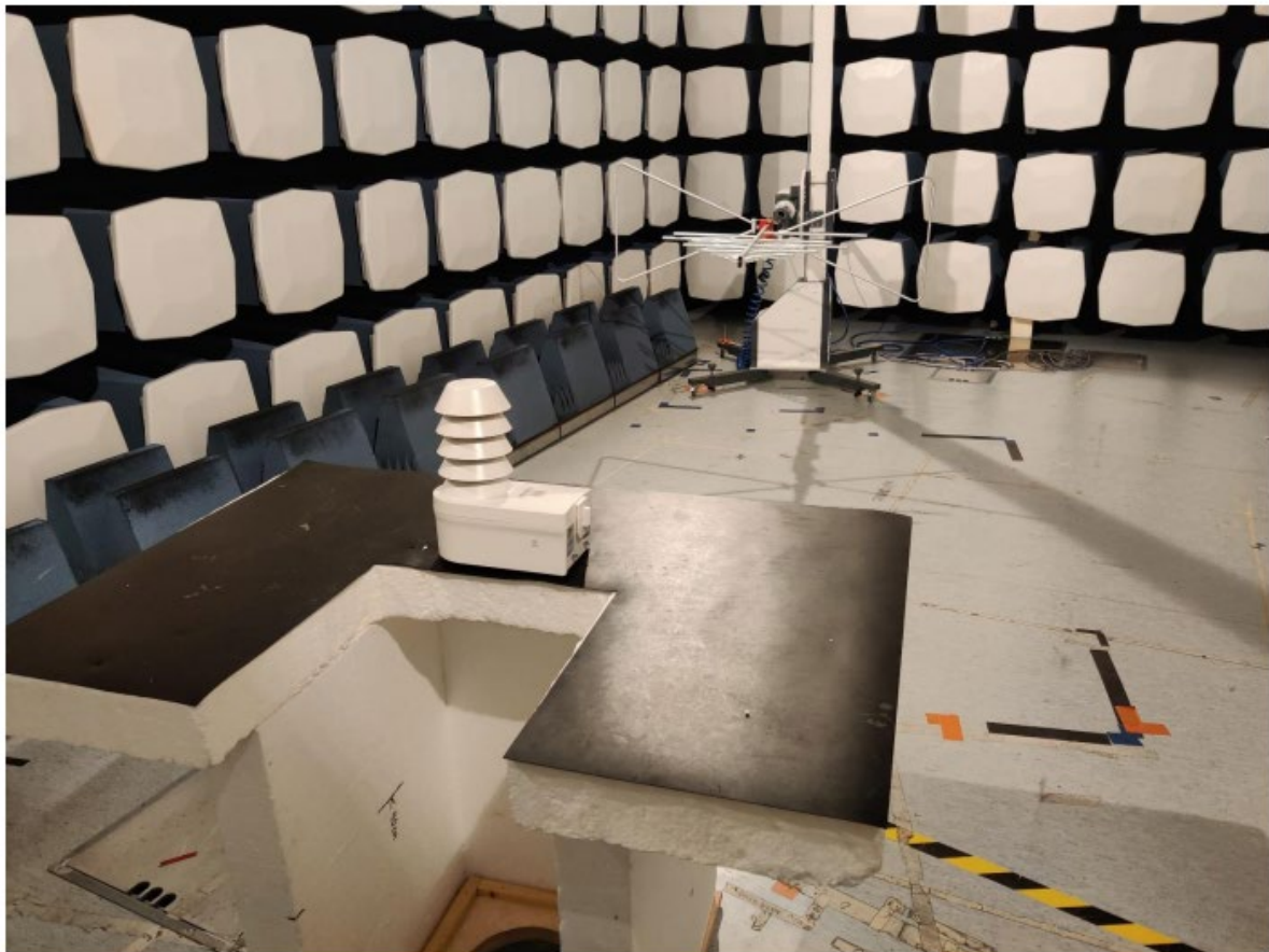
Picture 5 Radiated emission, 30 – 1000 MHz, common setup
