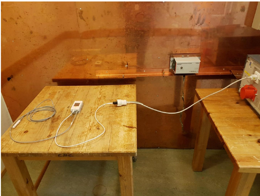
Test set up conducted emission 150 kHz – 30 MHz
