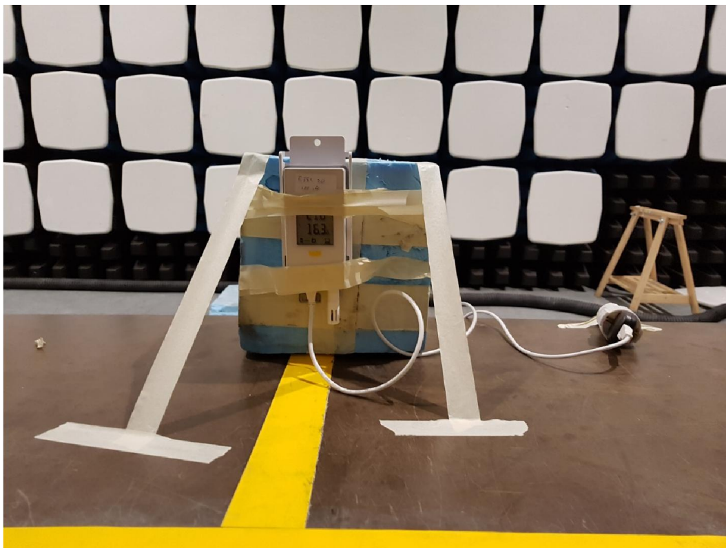
Test set up radiated emission
