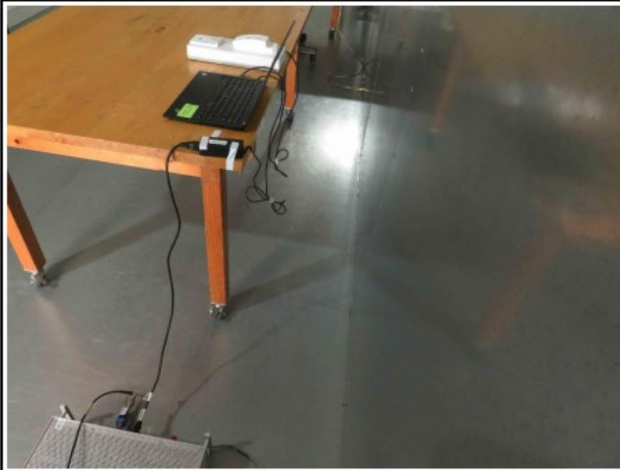
AC Powerline Setup-view 2
