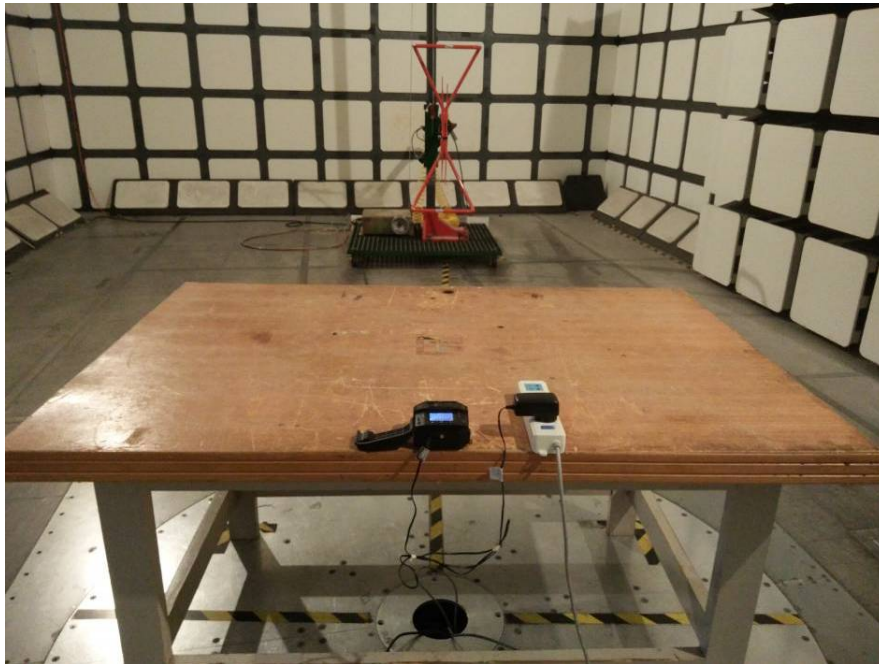
Radiated Emissions – Rear View (Below 1 GHz, Charging & Recording)
