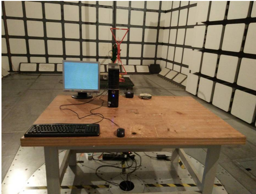
Radiated Emissions – Front View (Below 1 GHz, Downloading)
