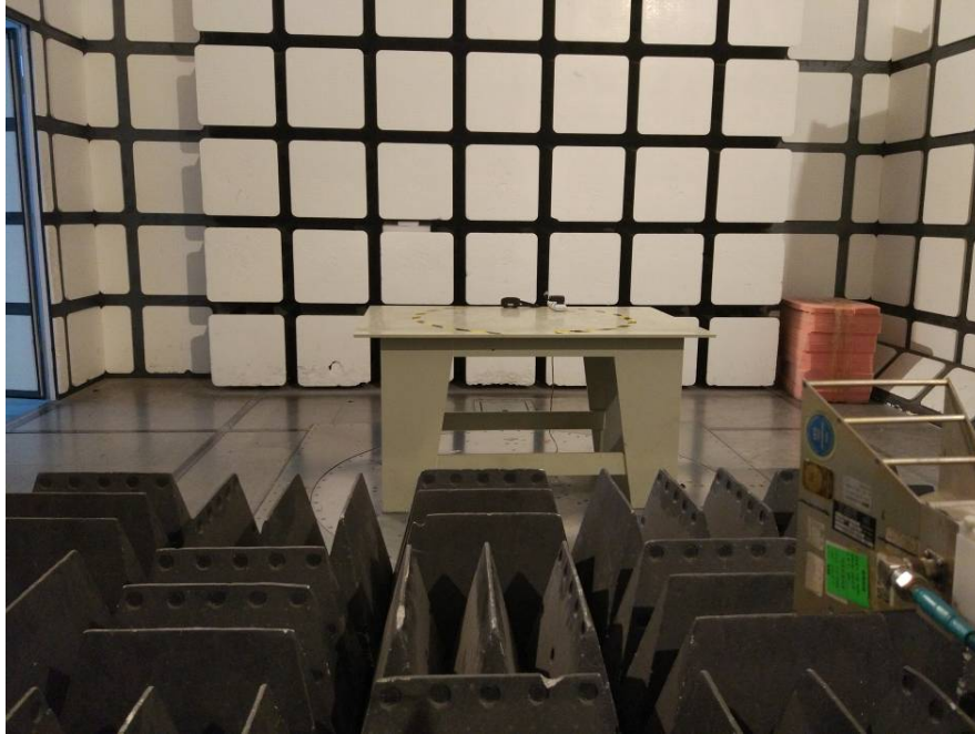
Radiated Emissions – Front View (Above 1 GHz, Charging & Recording)
