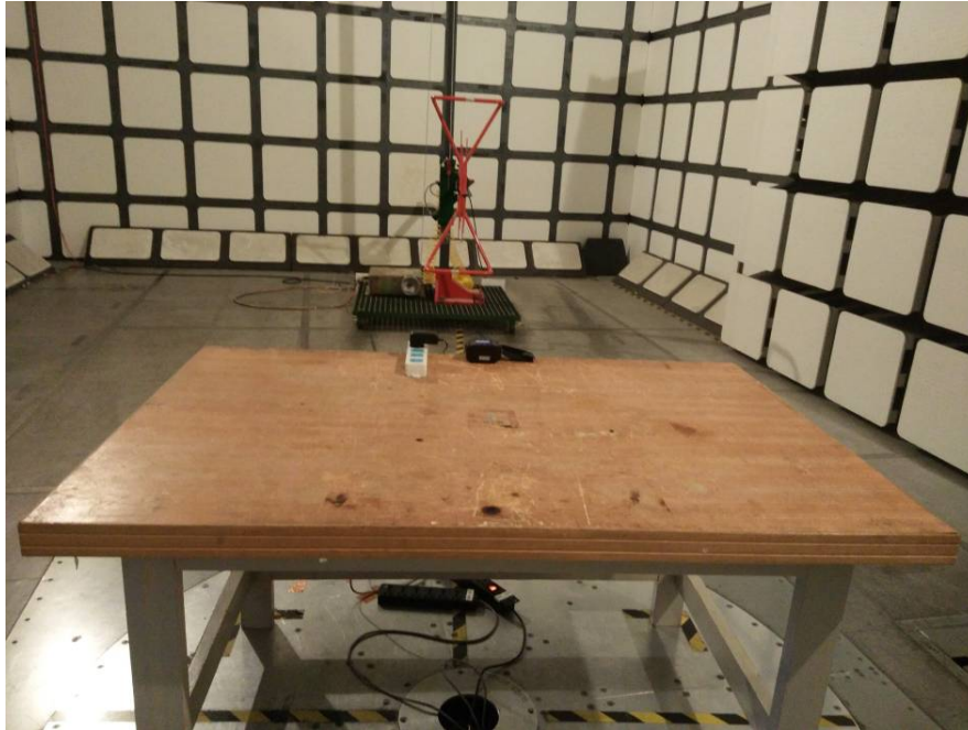
Radiated Emissions – Front View (Below 1 GHz, Charging & Recording)
