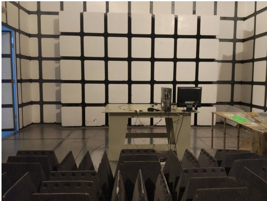
Radiated Emissions – Rear View (Above 1 GHz, Downloading)
