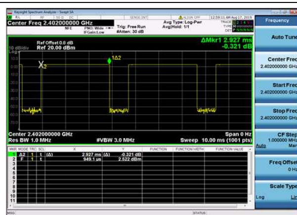
GFSK,2402,DH5,Transmission Time
