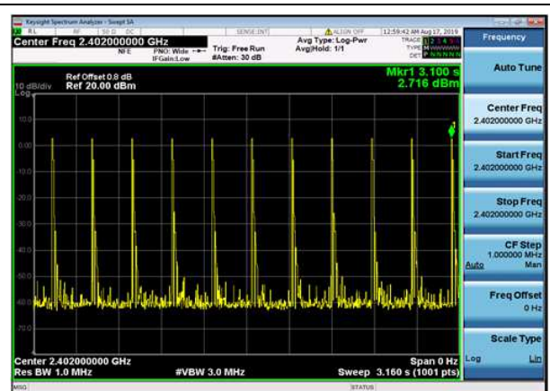
GFSK,2402,DH5,Transmission Number
