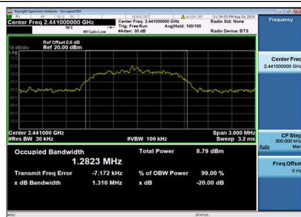
DQPSK,2441MHz,2DH5
