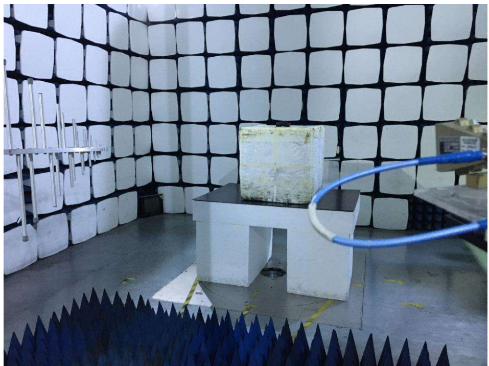
Radiation Emission Test Setup (Above 18 GHz)
