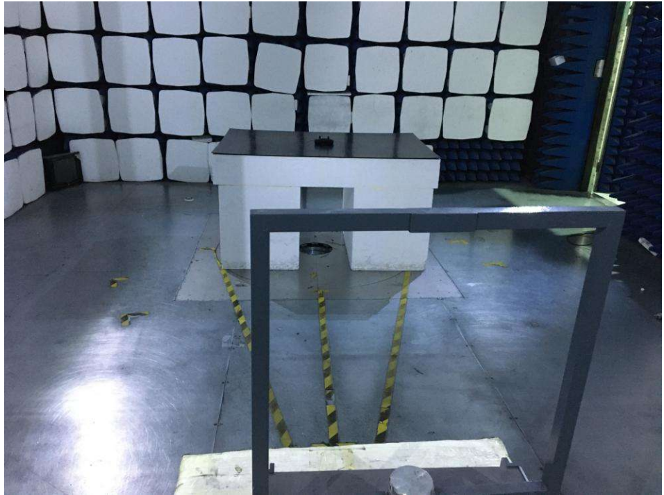
Radiation Emission Test Setup (Below 30 MHz)
