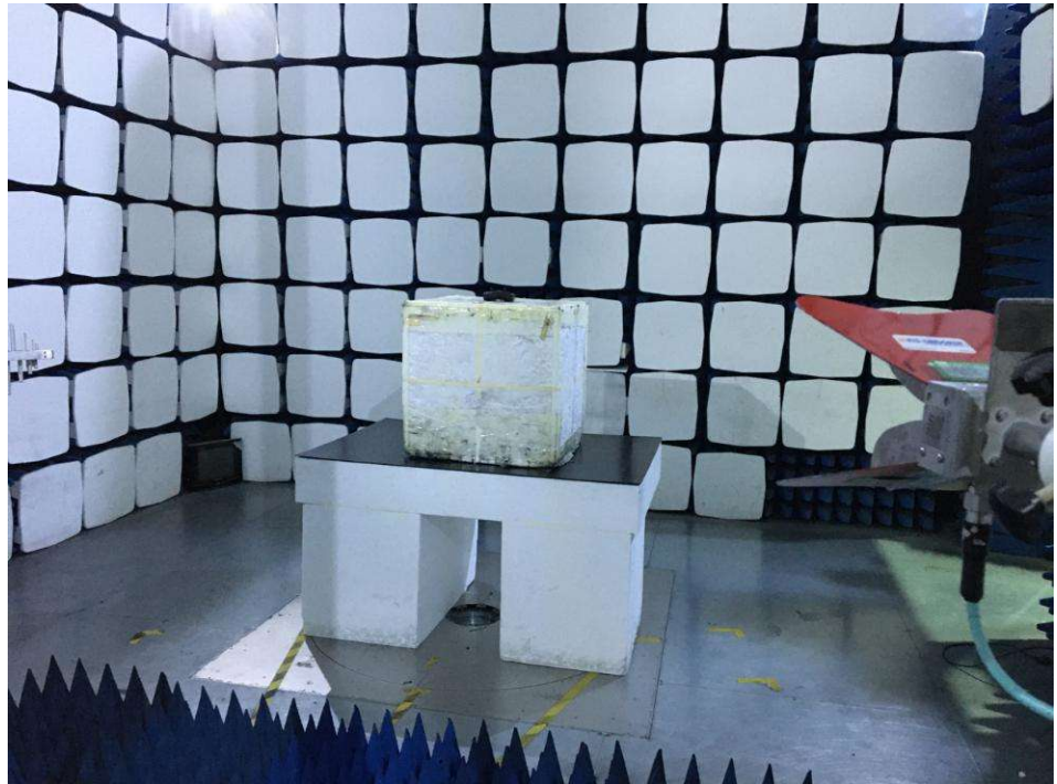
Radiation Emission Test Setup (1 GHz to 18 GHz)
