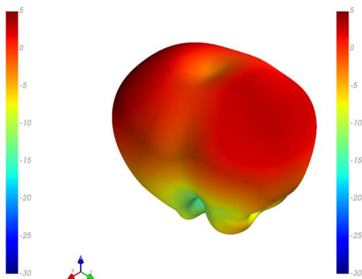
A40 Passive Ground Plane
