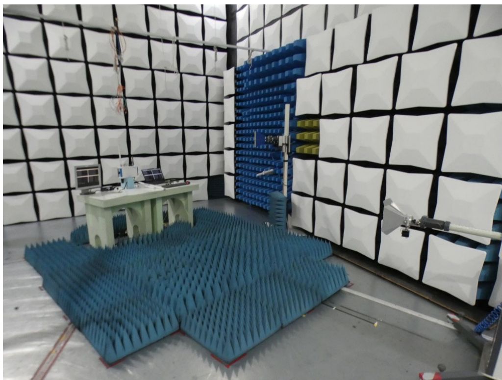
Photo 3: Test setup for radiated measurements (computer peripheral setup, 1 GHz – 18 GHz; unintentional radiator §15.109, ANSI C63.4)
