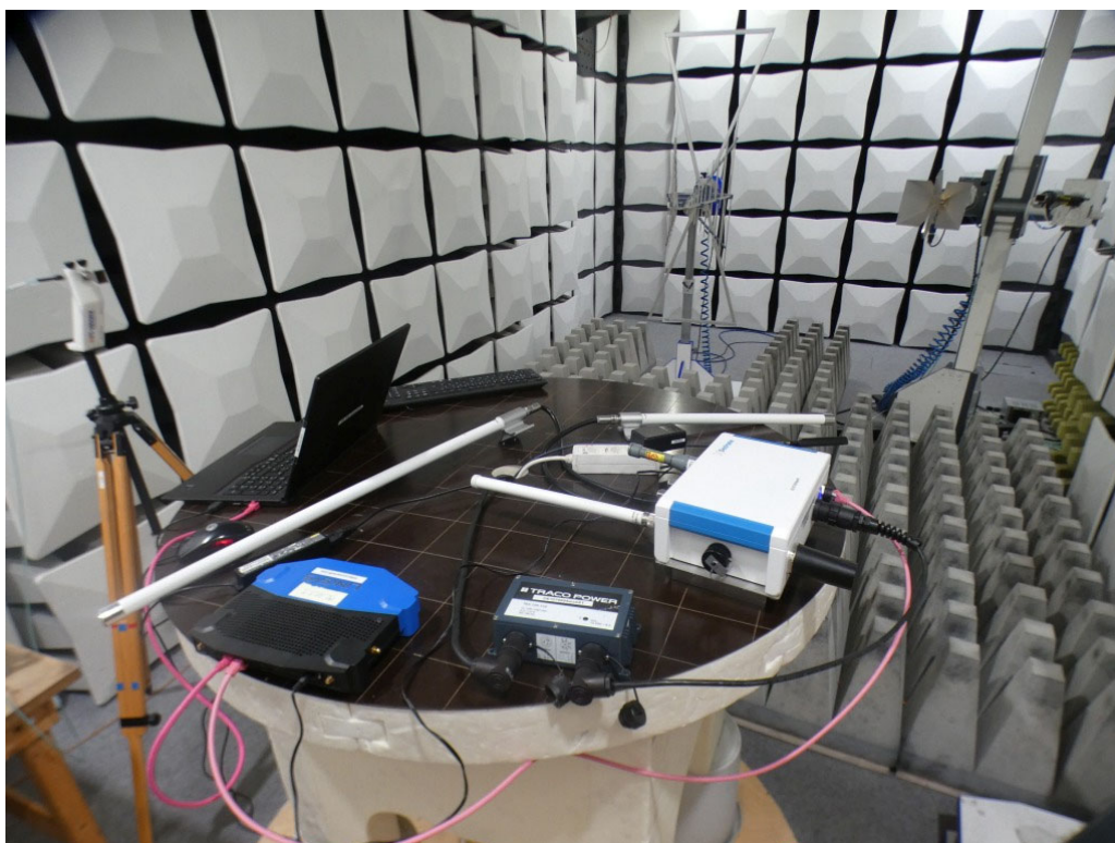
Photo 4: Test setup for radiated measurements (computer peripheral setup, 18 - 26 GHz; unintentional radiator §15.109, ANSI C63.4)
