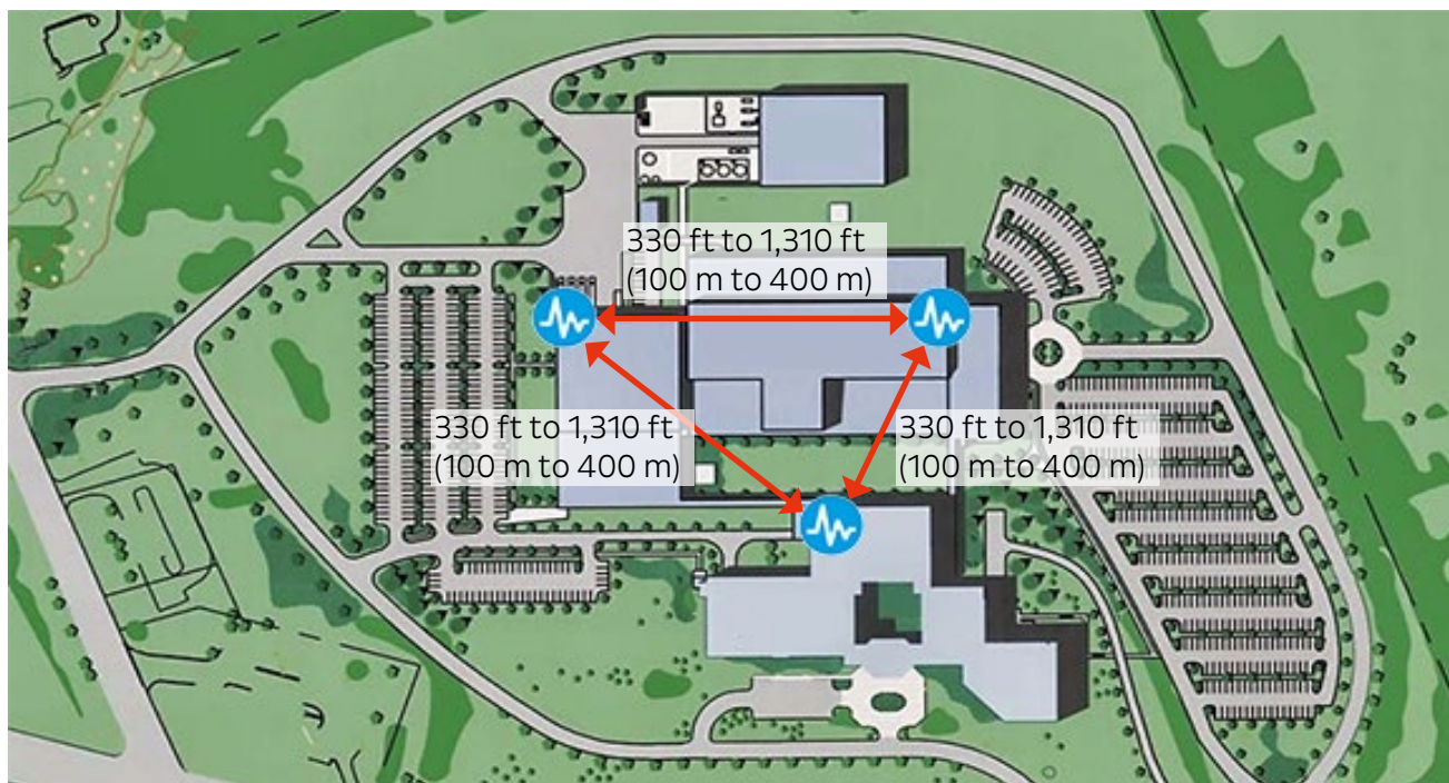
Distance between the RF-300s
