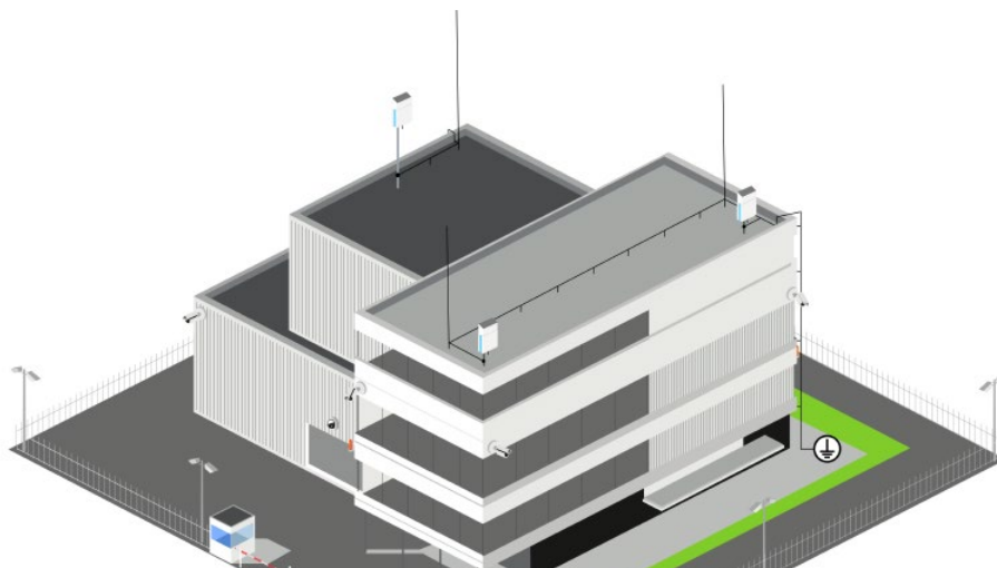
Lightning Protection Installation with RF-300s
