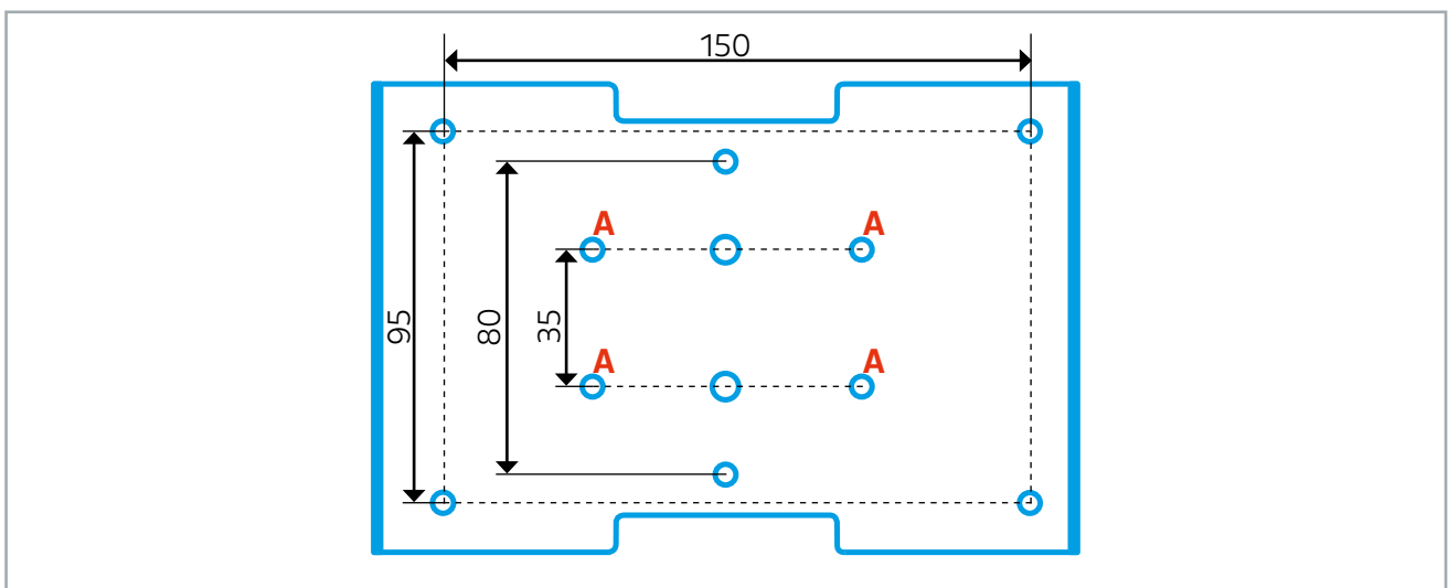
Dimensioning of the holes of the RF Mounting Plate
