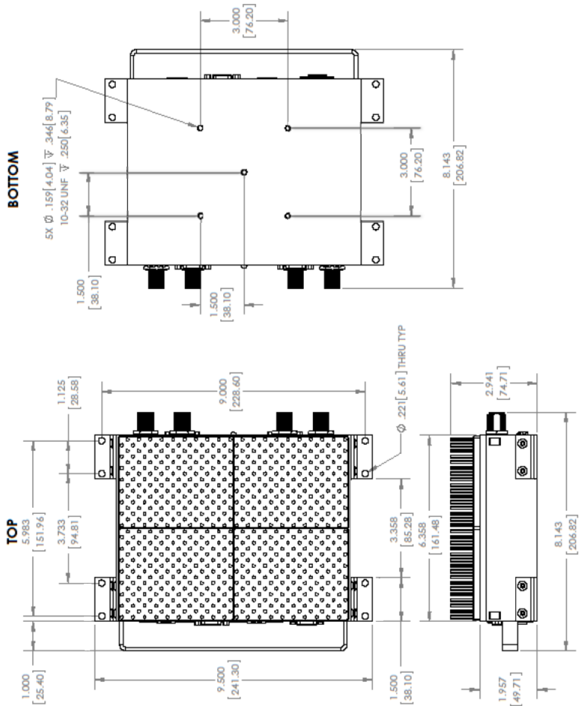
Figure 6 Mounting Dimensions – Standalone Unit
