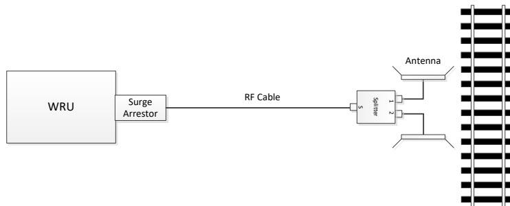
Figure 8 Access Point Radio Installation – Two Antennas
