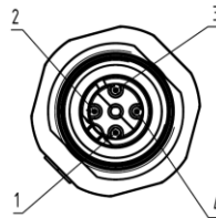
Figure 3 Ethernet Port Pin-out
