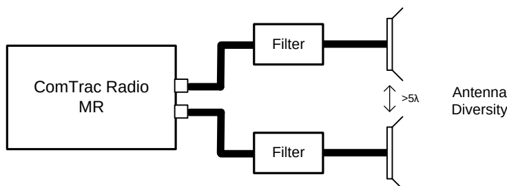
Figure 10 Mobile Radio Installation
