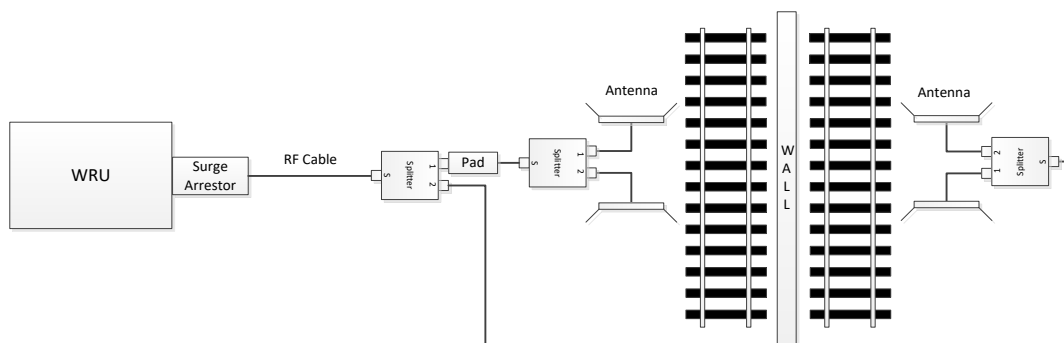
Figure 9 Access Point Radio Installation – Four Antennas
