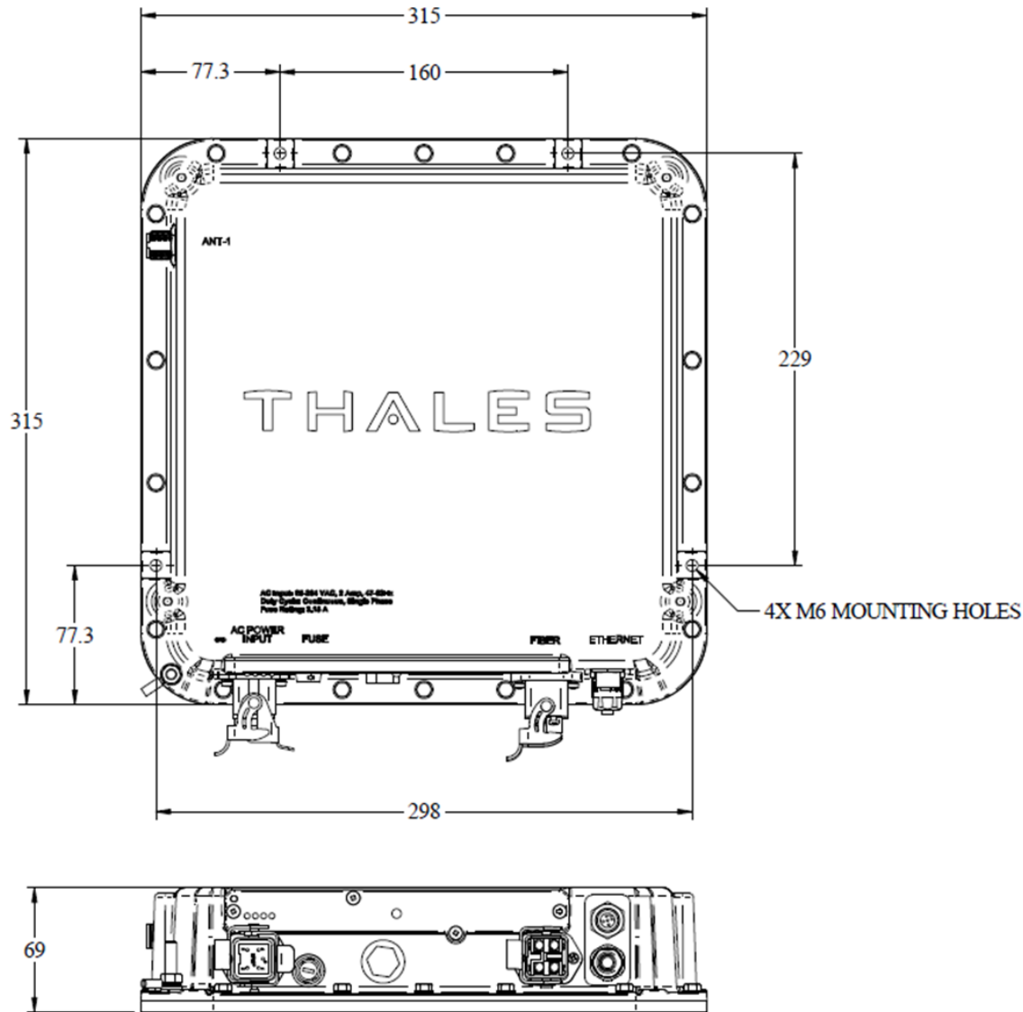
Figure 7 Mounting Dimensions – Die-cast Unit
