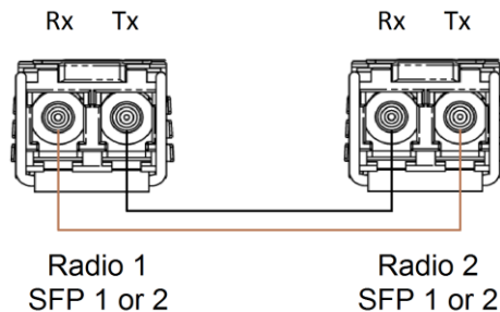
Figure 2 Fibre Port Connection
