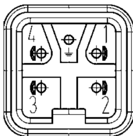
Figure 5 Power Port Pin-out
