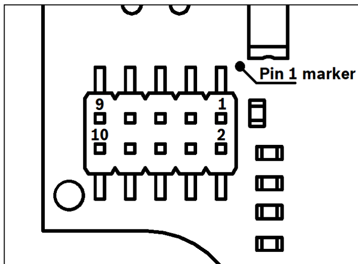
Figure 4 Debugger connector
