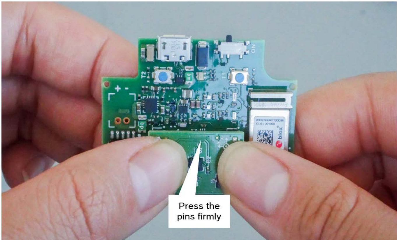
Figure 9 Connecting the Shuttle Board 3.0
