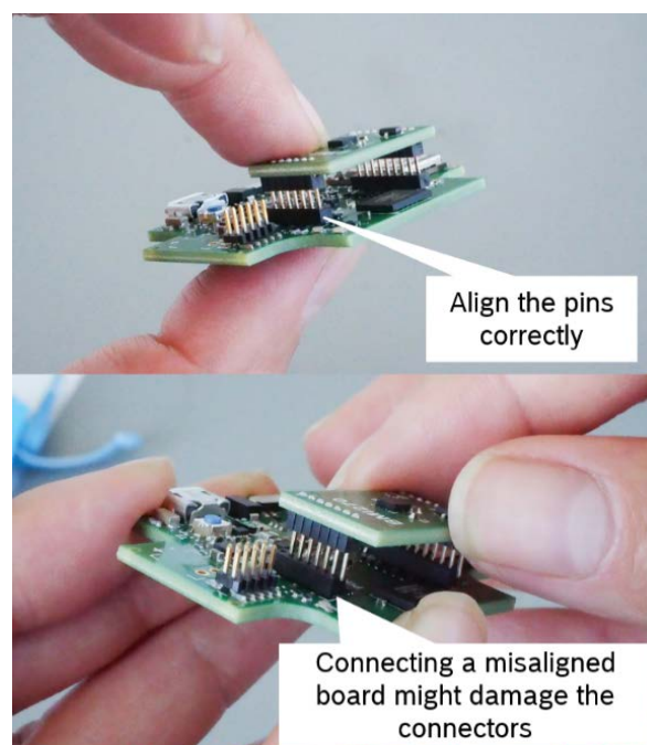
Figure 8 Aligning the pins of the Shuttle Board 3.0 board
