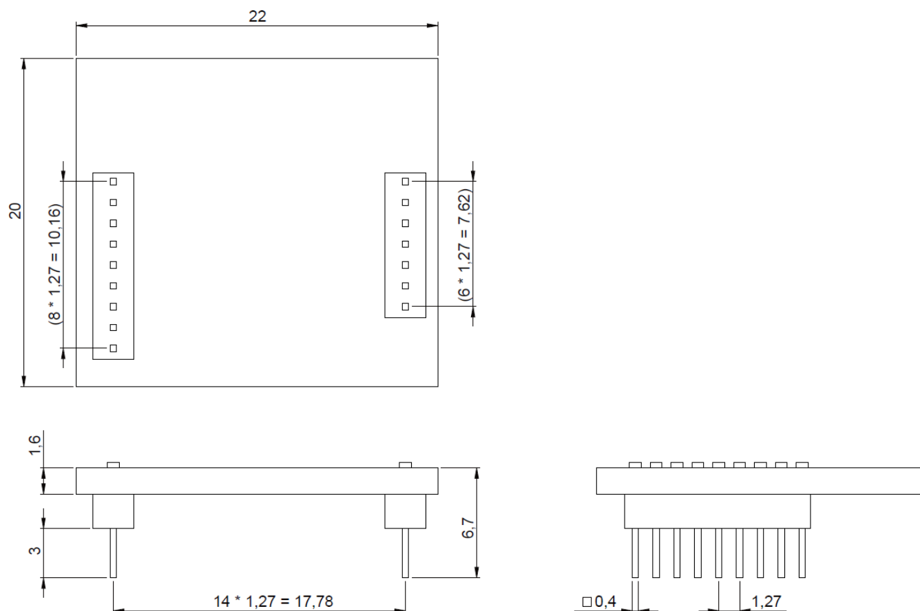
Figure 6 Multi-sensor Shuttle Board 3.0 dimensions
