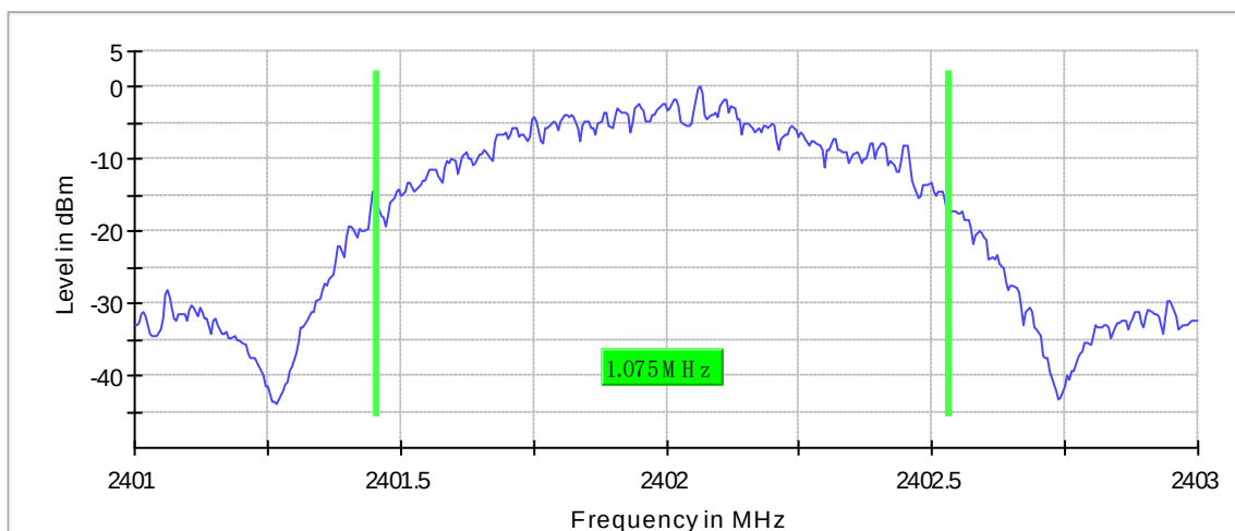
99 % Bandwidth
