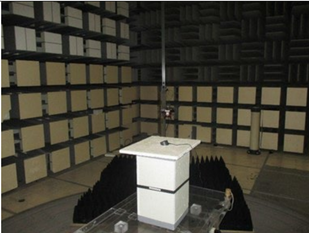
Radiated Emissions, 1GHz to 18GHz
