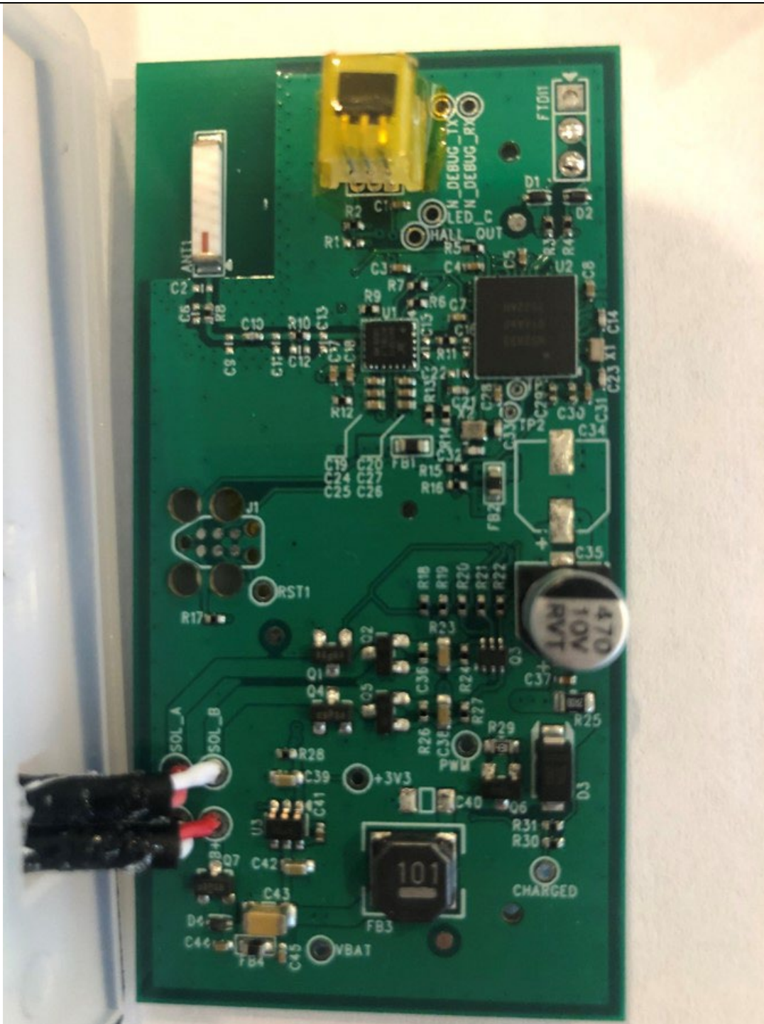
PCB Detail View (Top View)
