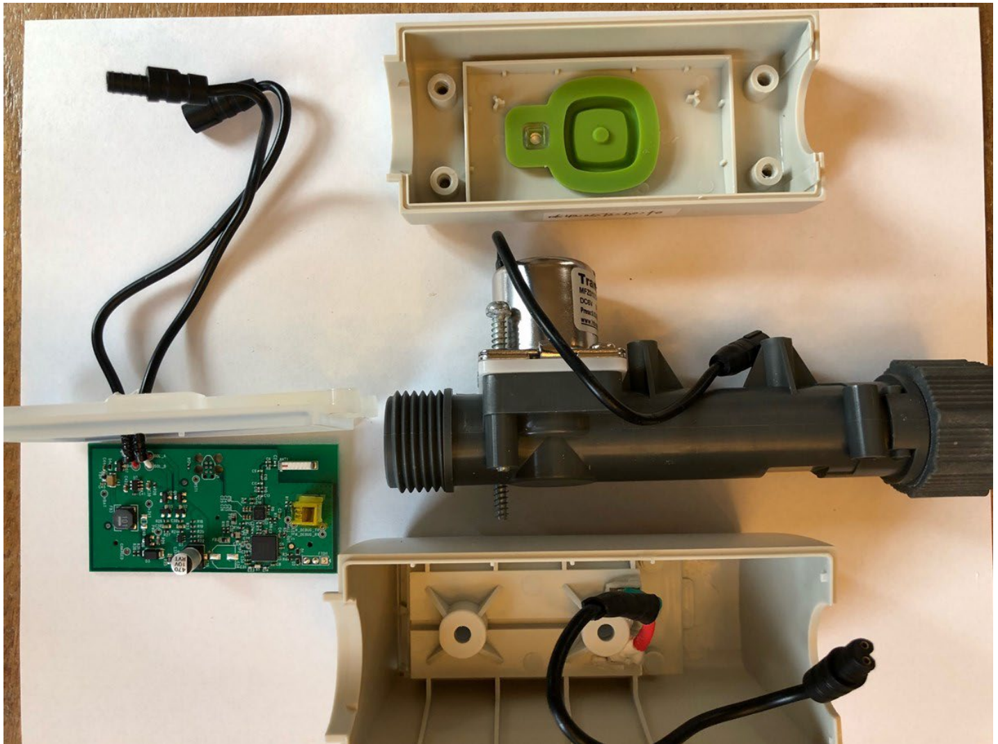
Exploded View
