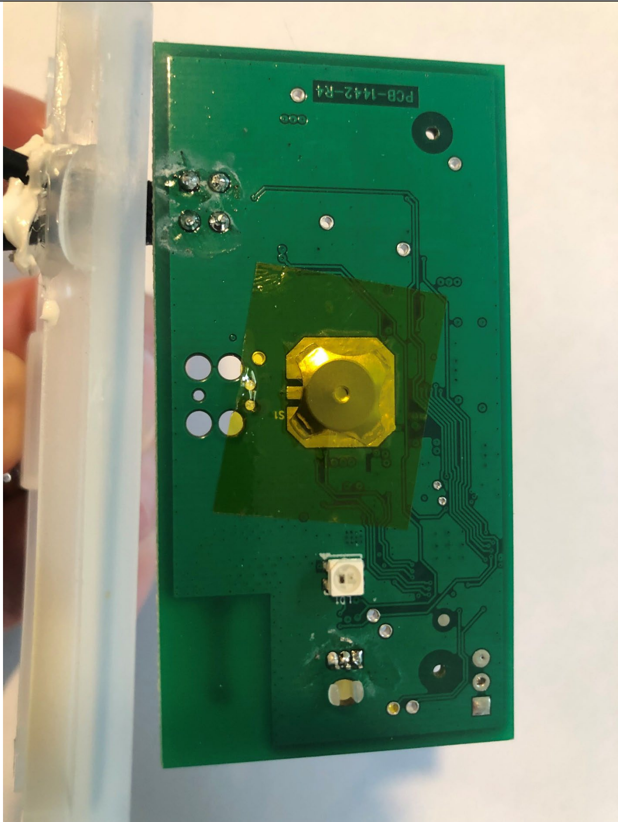
PCB Detail View (Bottom View)
