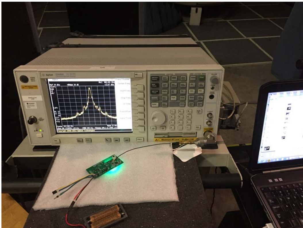
Conducted Antenna Port Measurements; Power, PSD, Bandwidth
