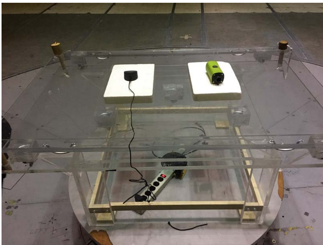
Radiated Emissions; Spurious; with Companion Device; Back
