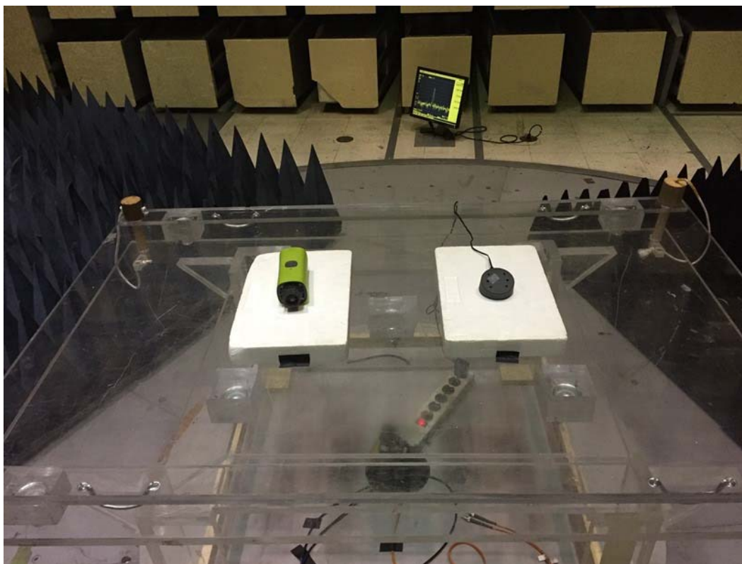
Radiated Emissions; Spurious; with Companion Device; Front
