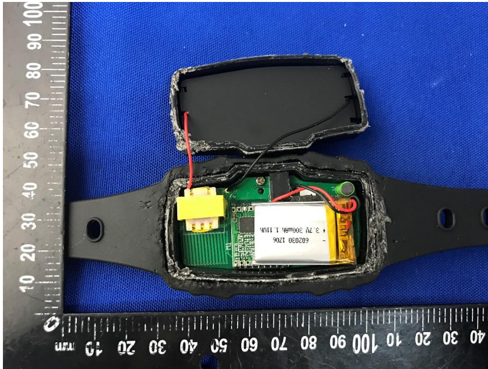
EUT UNCOVER VIEW (Receiver)
