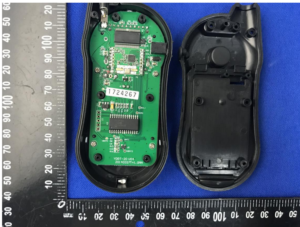
EUT UNCOVER VIEW (Remote Control)
