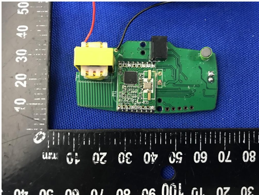
MAIN BOARD TOP VIEW (Receiver)
