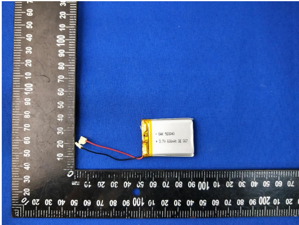
Battery Photo (FRONT) (Remote Control)
