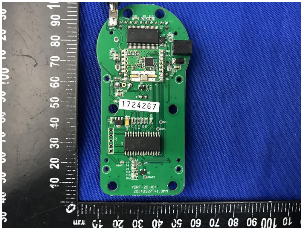
MAIN BOARD TOP VIEW (Remote Control)
