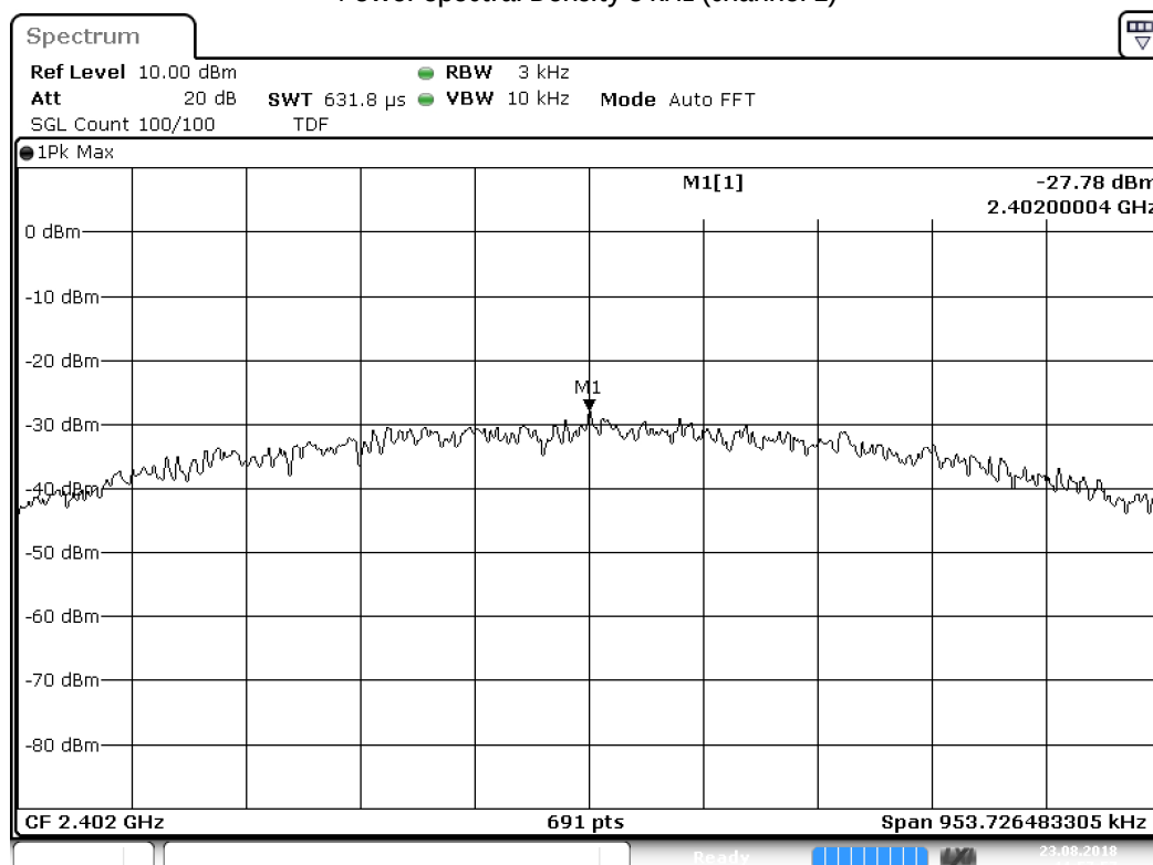
Power Spectral Density 3 kHz (channel 1)
