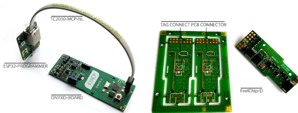
Figure 1 - ESP32 Programmer
