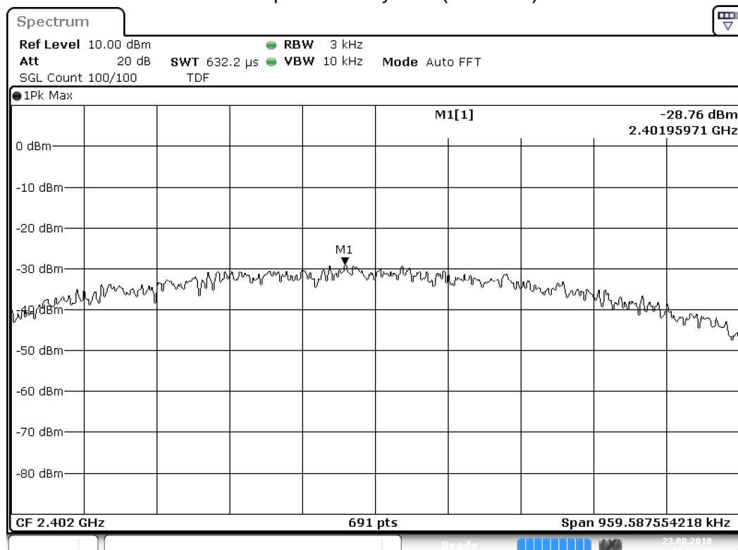
Power Spectral Density 3 kHz (channel 37)
