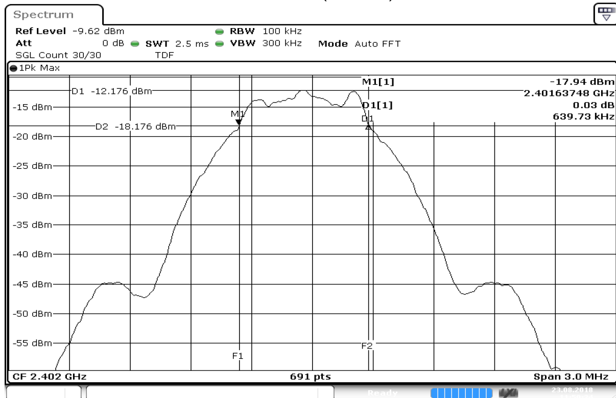
6 dB Bandwidth (Channel 37)
