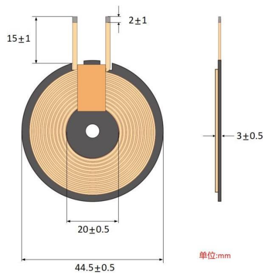
Model drawing
