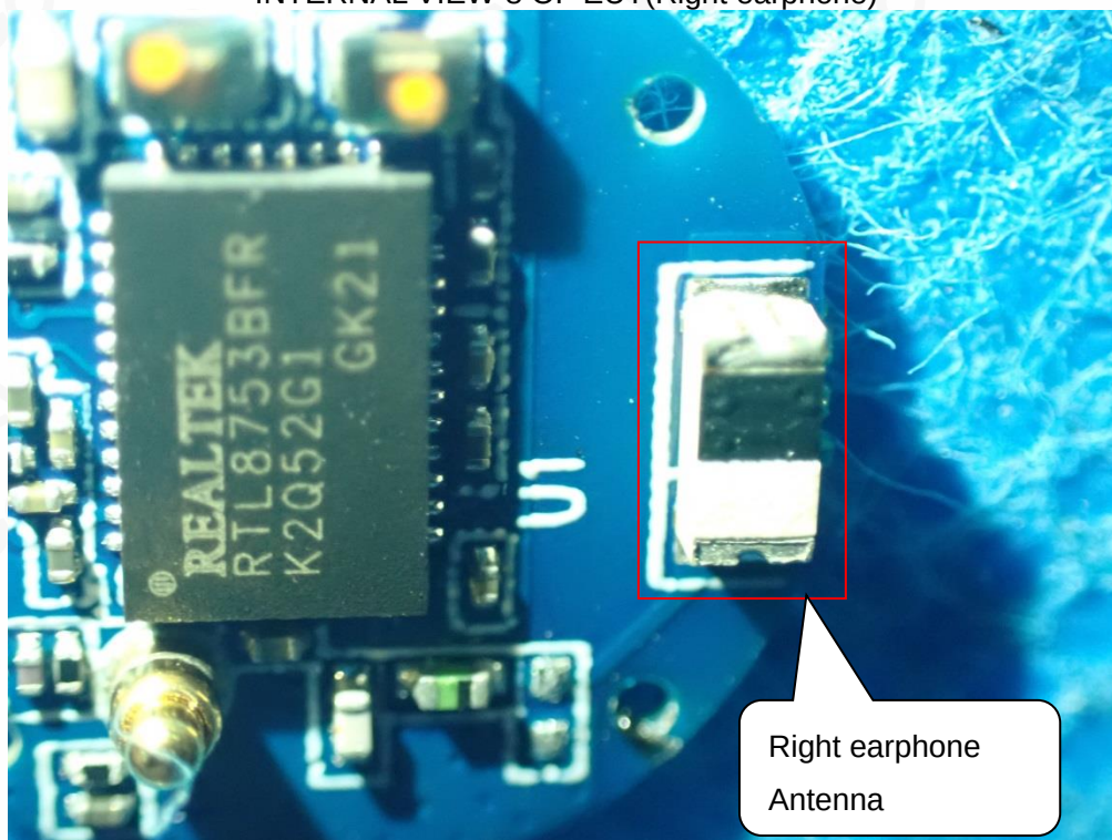
INTERNAL VIEW-8 OF EUT(Right earphone)
