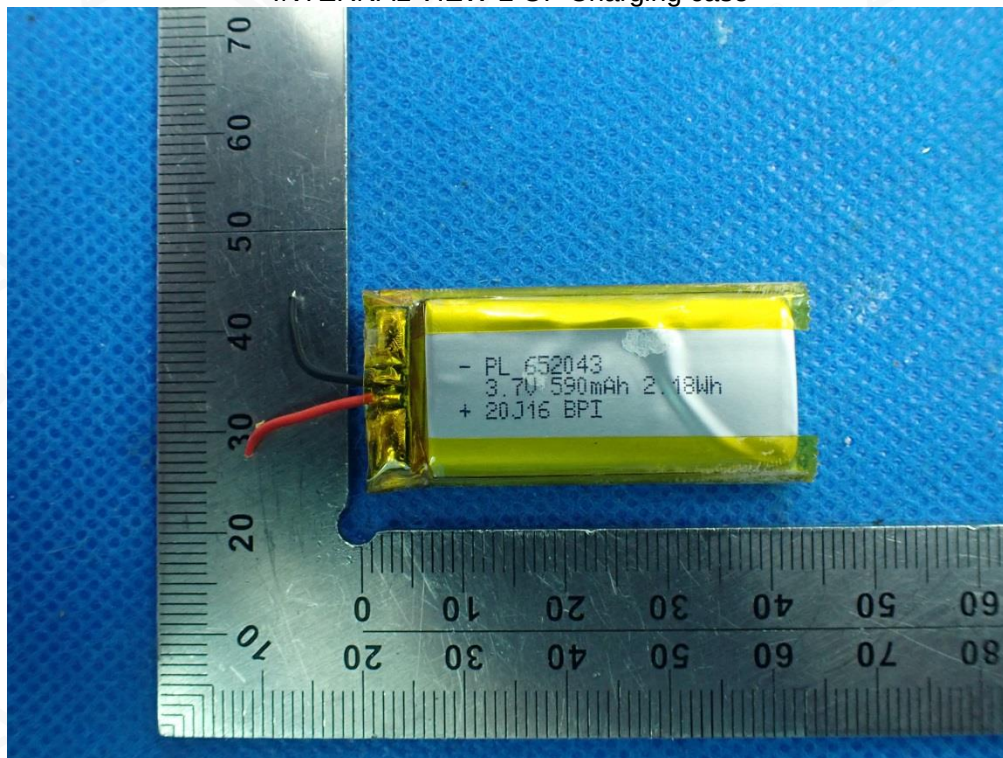
INTERNAL VIEW-2 OF Charging case
