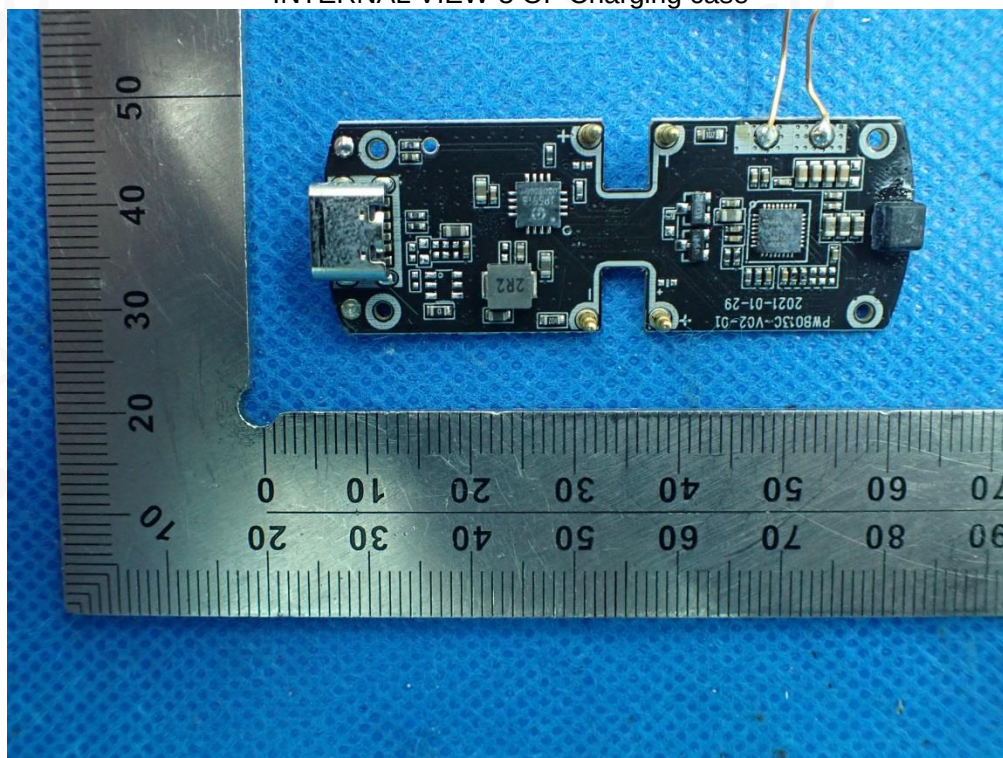
INTERNAL VIEW-3 OF Charging case
