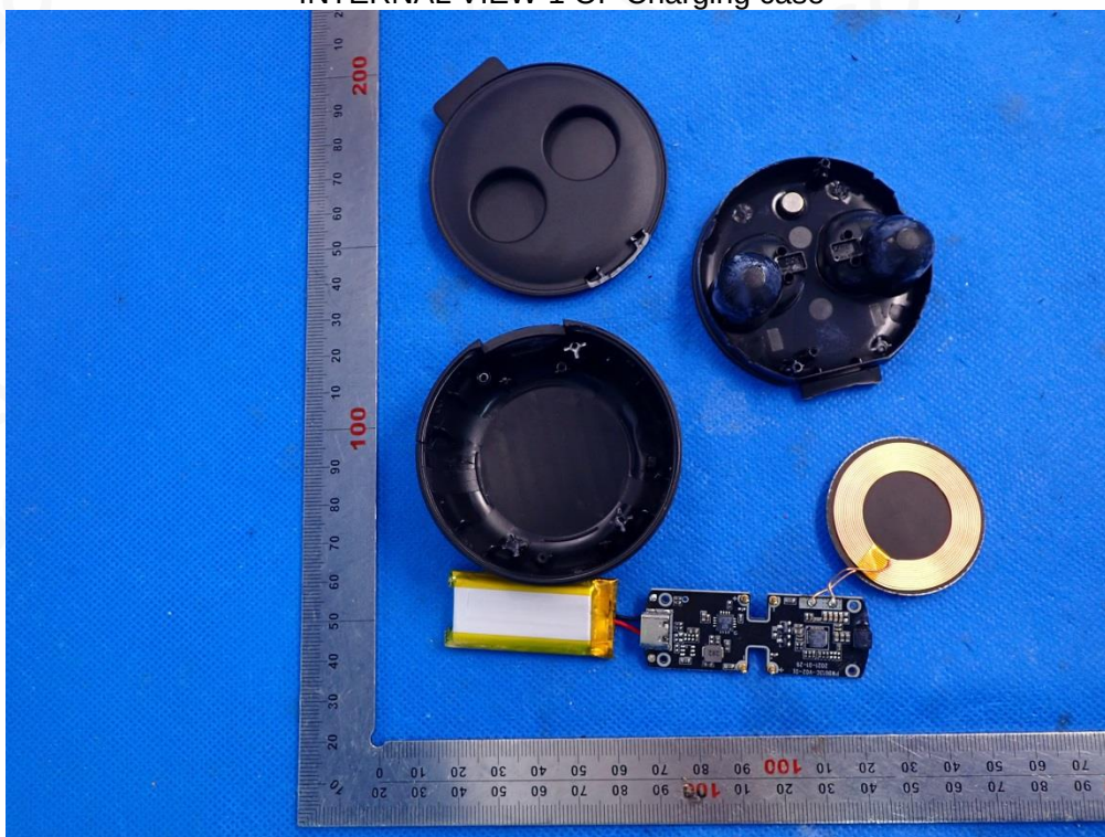
INTERNAL VIEW-1 OF Charging case
