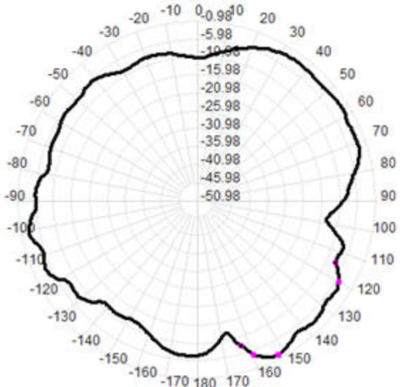
2460.0MHz Total(E2), Max= -2.40dBi
