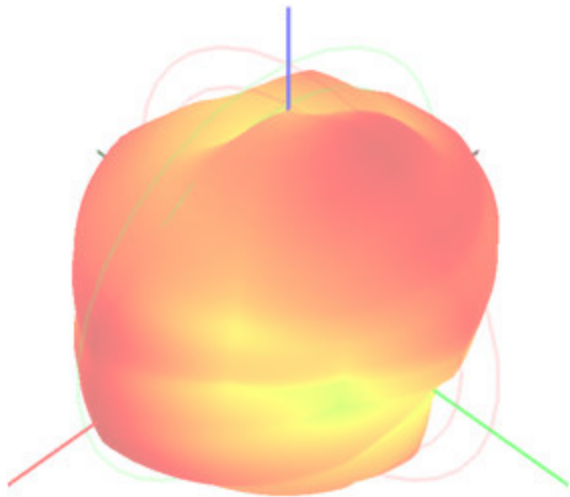
2460.0MHz H+V, Eff: 20.6%
