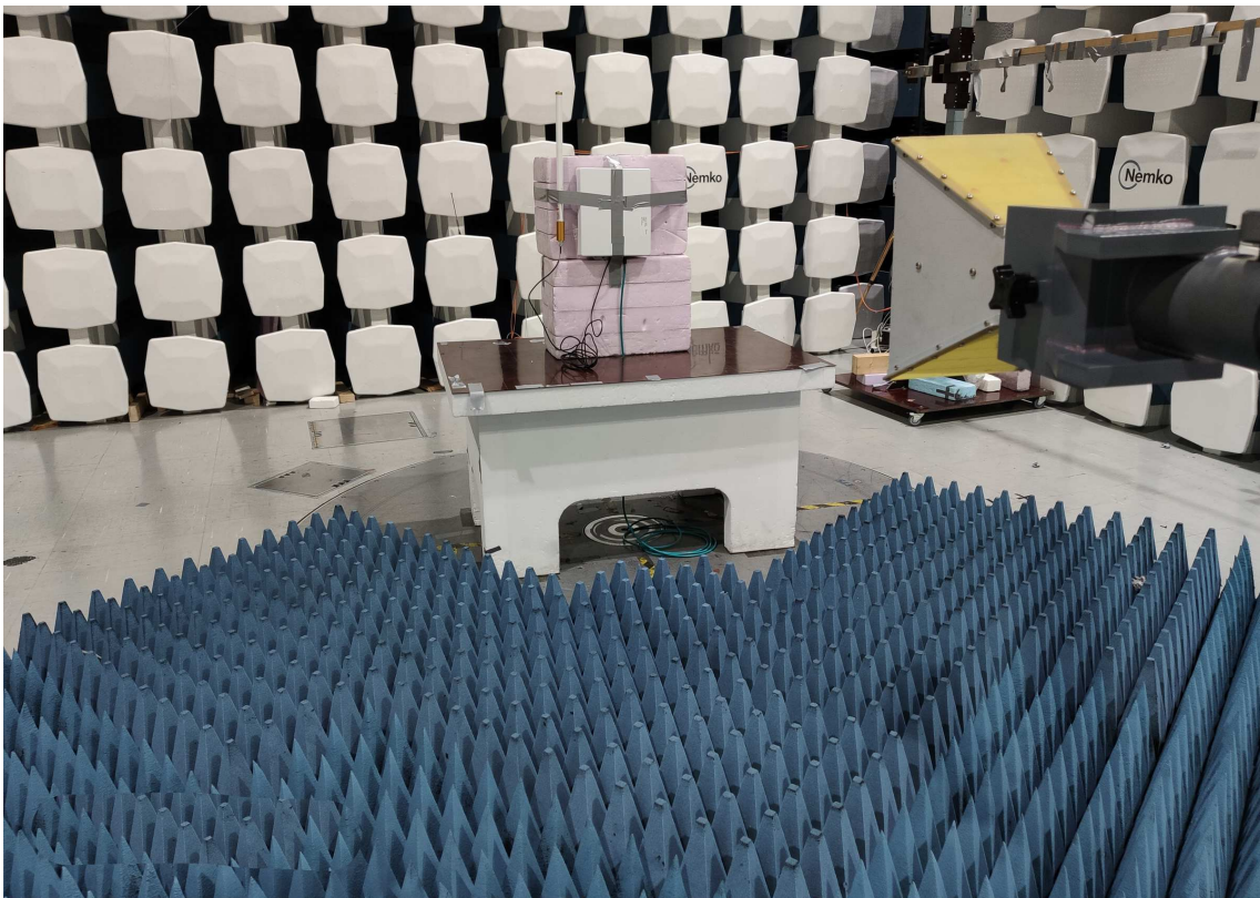
Radiated Emissions, 1-10 GHz
