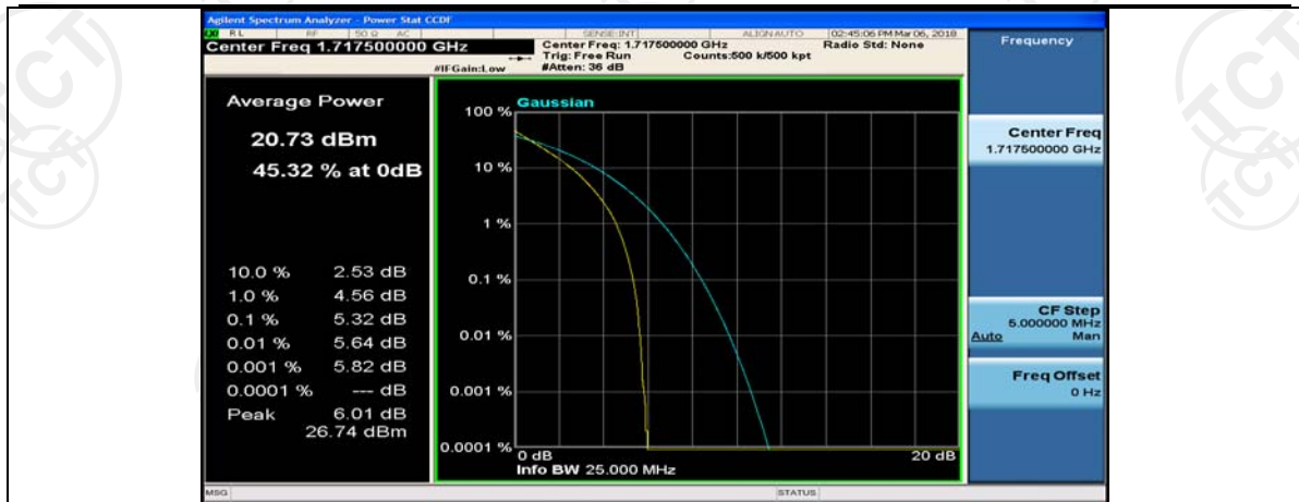
(Channel Bandwidth:15 MHz)_MCH_QPSK_1RB#0
