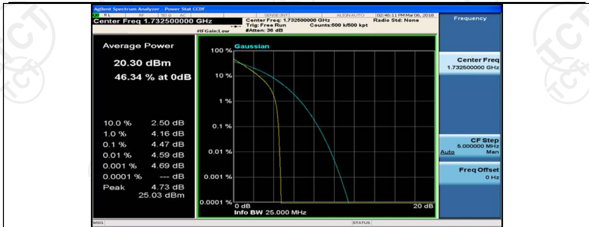
(Channel Bandwidth:15 MHz)_MCH_QPSK_75RB#0
