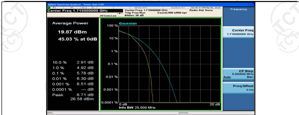
Channel Bandwidth: 10 MHz_MCH_16QAM_1RB#0
