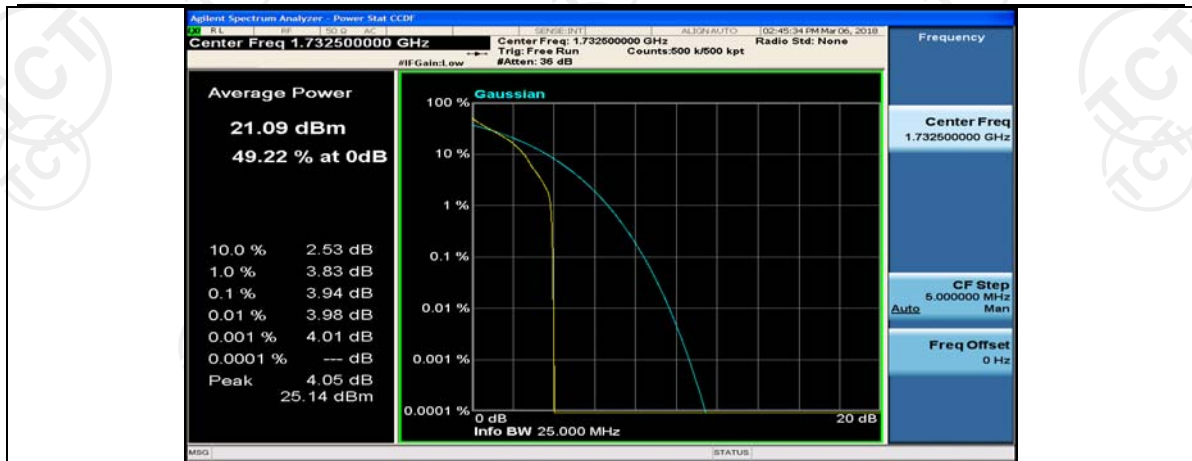
(Channel Bandwidth:15 MHz)_MCH_QPSK_37RB#0
