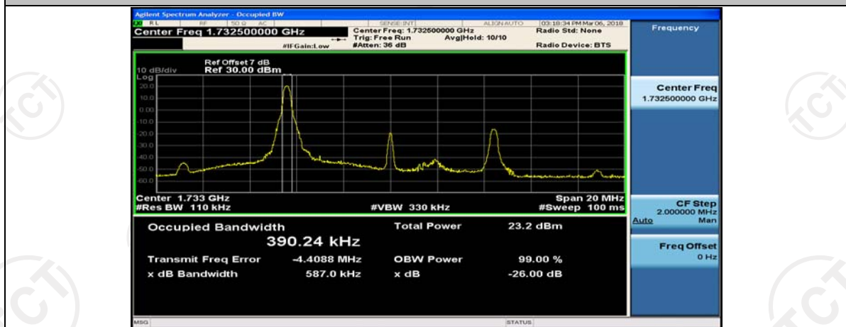
Channel Bandwidth: 10 MHz_MCH_QPSK_1RB#25
