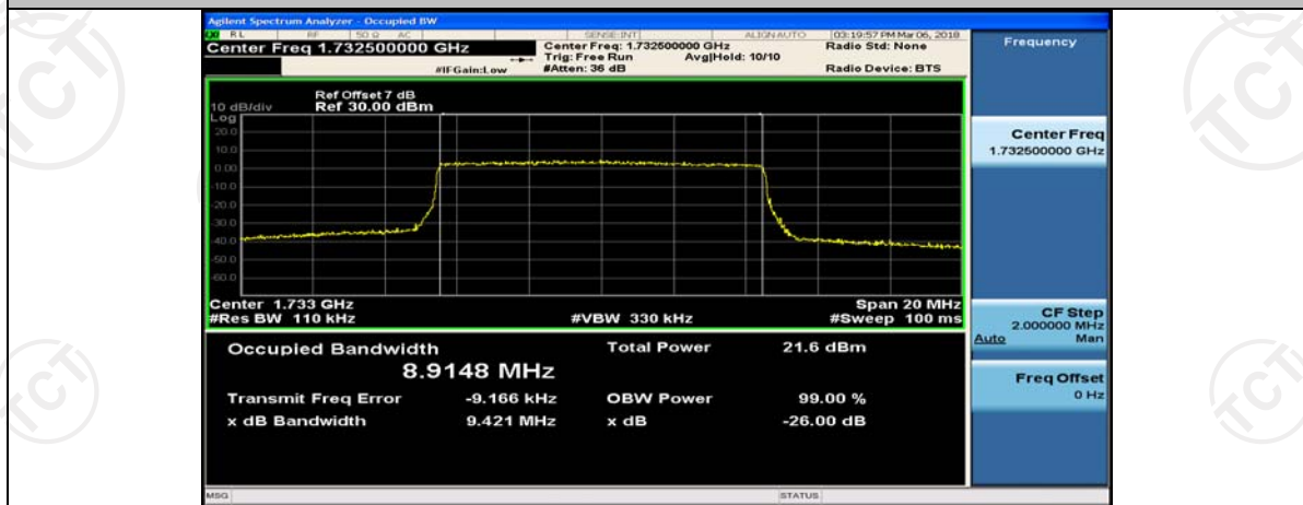
Channel Bandwidth: 10 MHz_MCH_16QAM_50RB#0
