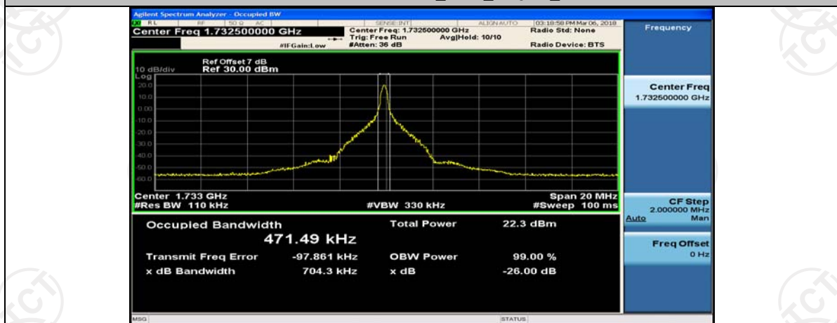
Channel Bandwidth: 10 MHz_MCH_16QAM_1RB#49
