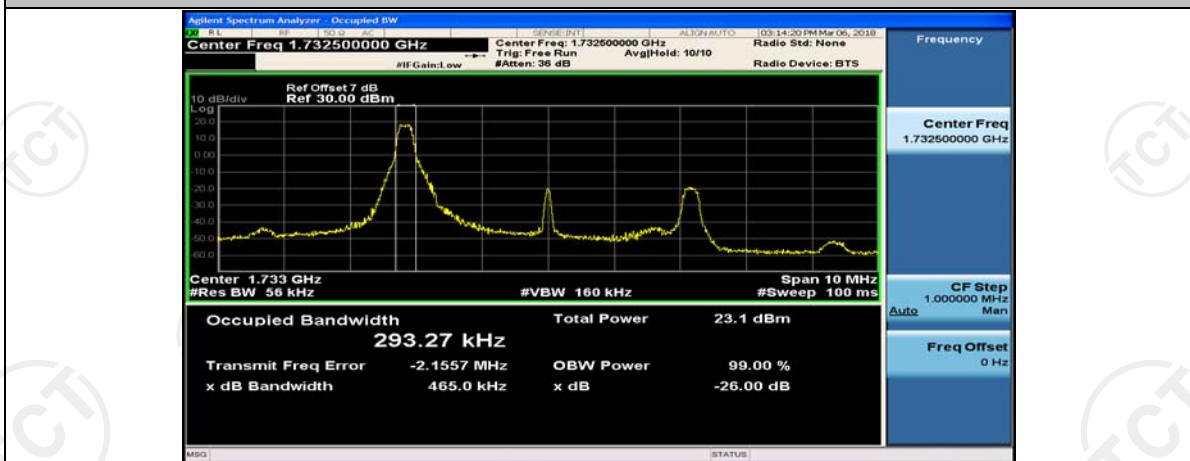
(Channel Bandwidth: 5 MHz)_MCH_16QAM_1RB#12
