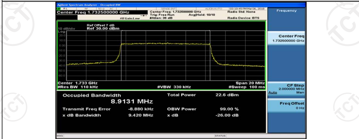
Channel Bandwidth: 10 MHz_MCH_QPSK_50RB#0
