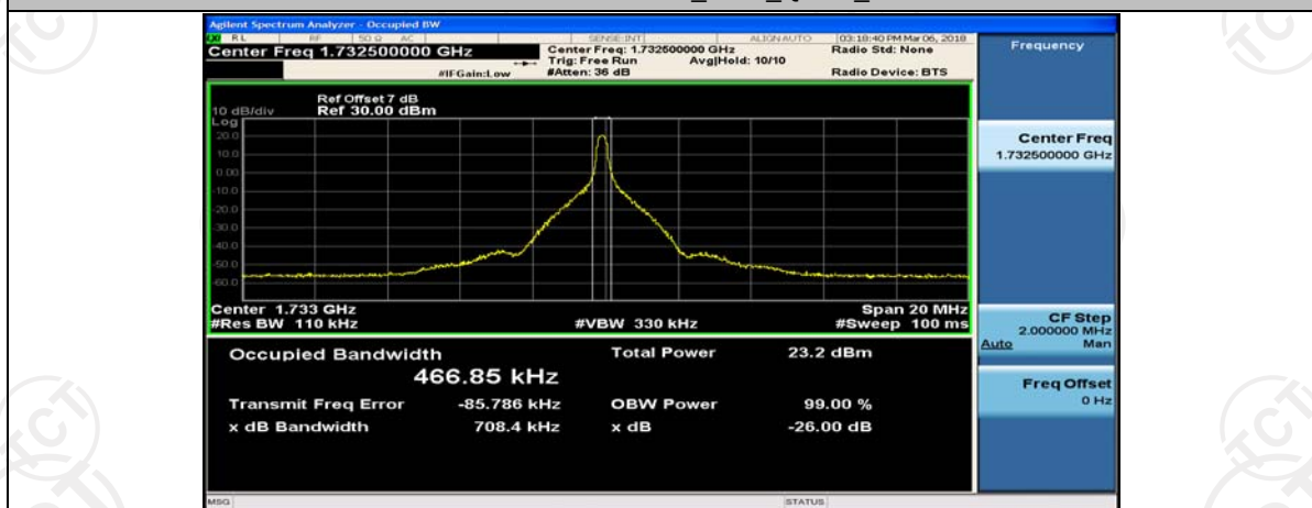
Channel Bandwidth: 10 MHz_MCH_QPSK_1RB#49
