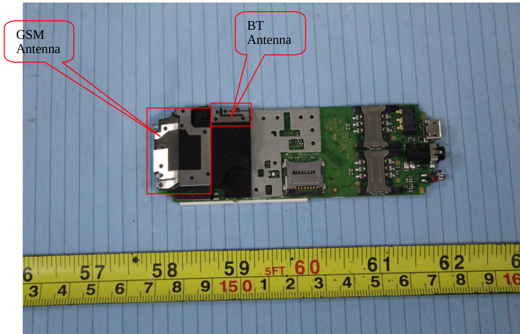
EUT – Main Board Bottom View 1
