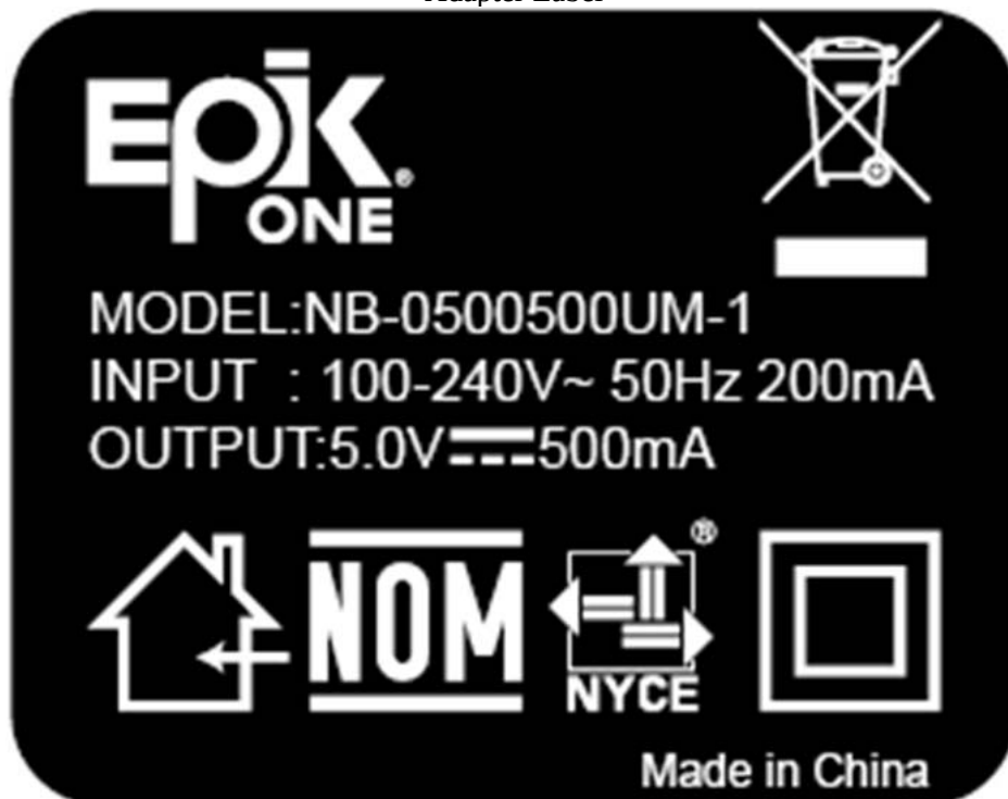
Adapter Label
