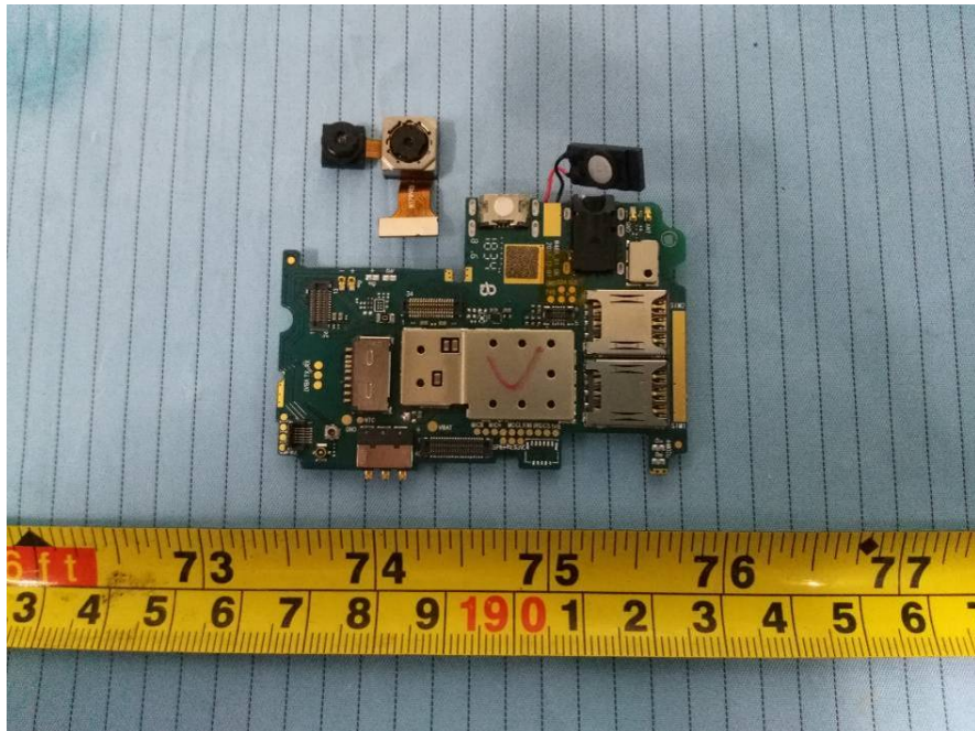
EUT – Main Board Top View 1(Model: 536)
