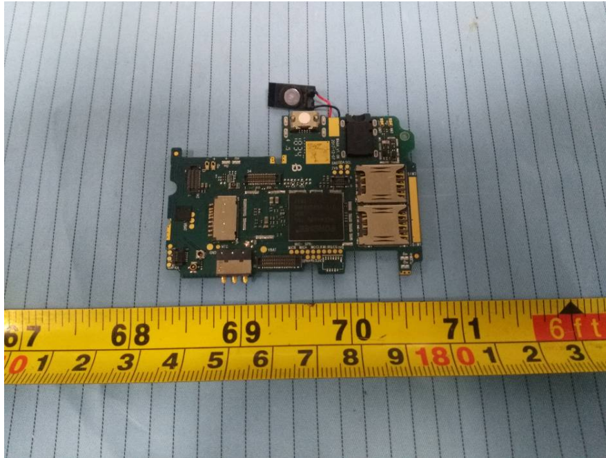
EUT – Main Board Top Shielding off View (Model: 535)
