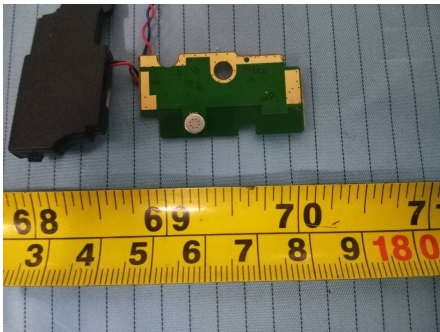
EUT –Small Board Bottom shield off View (Model: 535)
