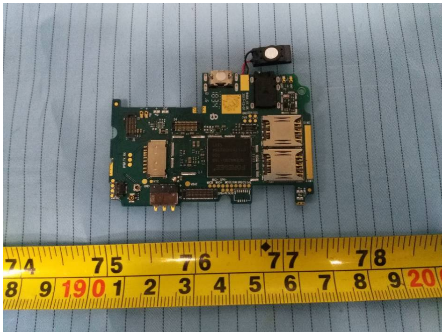
EUT – Main Board Top Shielding off View (Model: 536)
