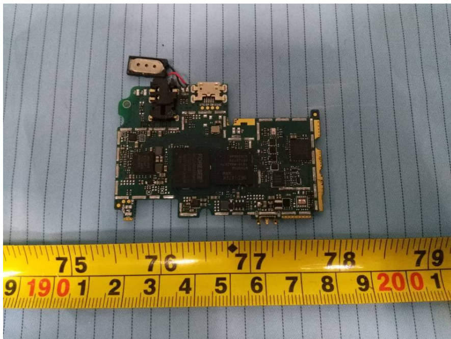
EUT – Main Board Bottom shield off View (Model: 536)
