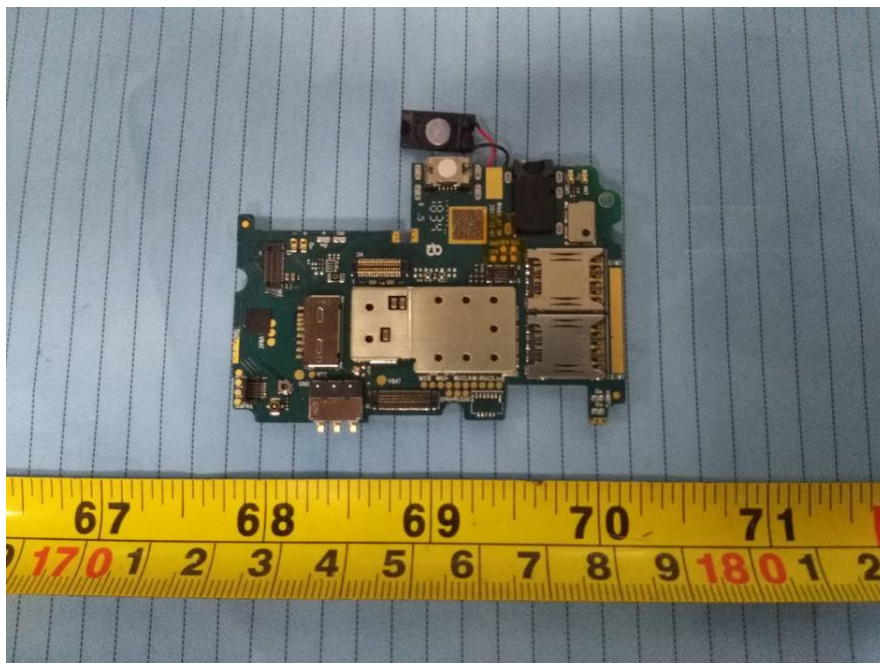
EUT – Main Board Top View 2(Model: 535)
