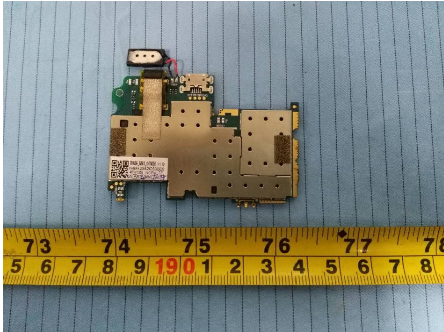
EUT – Main Board Bottom View (Model: 536)
