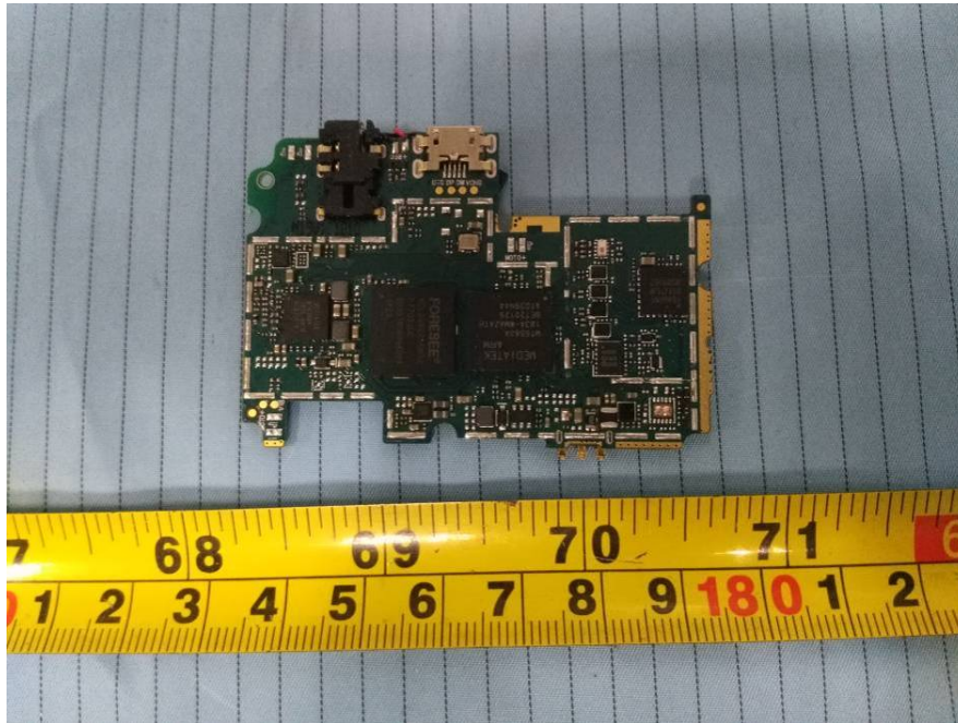
EUT – Main Board Bottom shielding off View (Model: 535)
