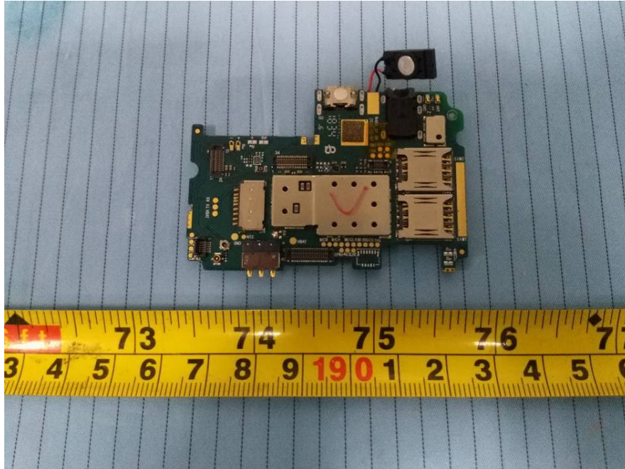
EUT – Main Board Top View 2(Model: 536)
