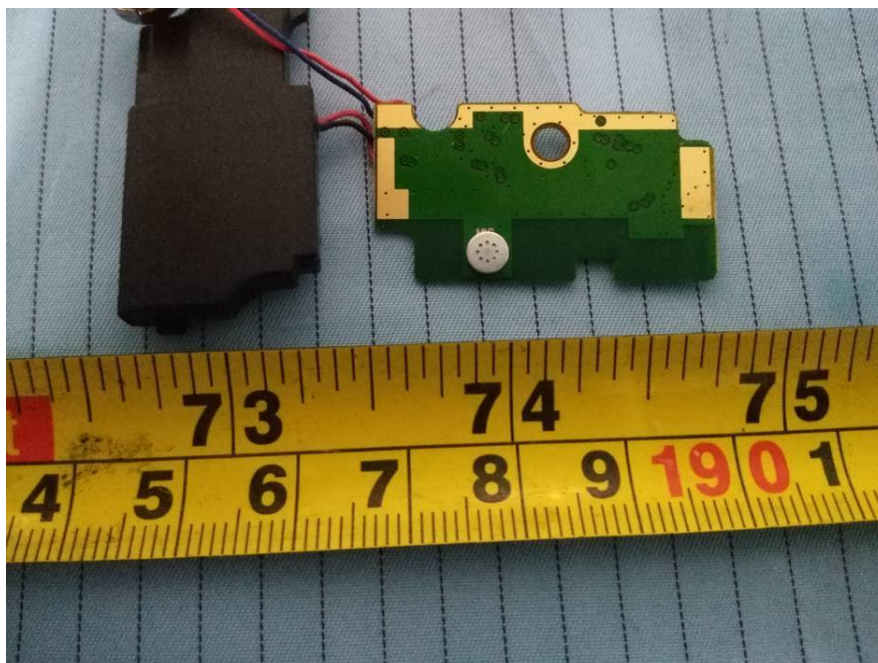
EUT –Small Board Bottom shield off View (Model: 536)
