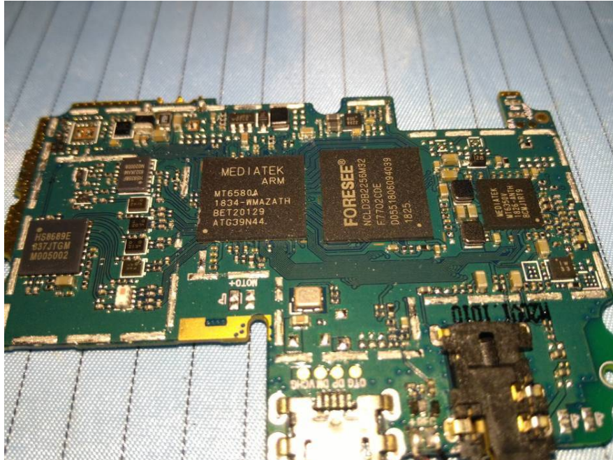
EUT – Main Chip View (Model: 536)
