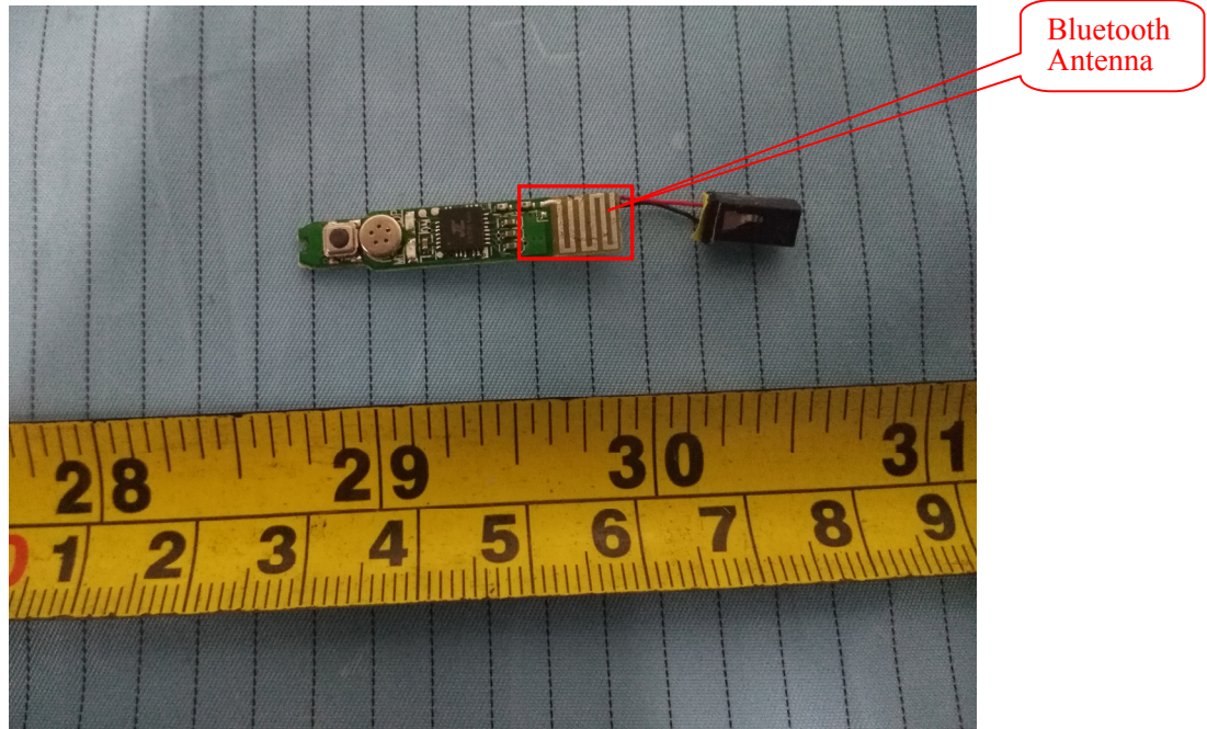
EUT –Main Board Bottom View 2
