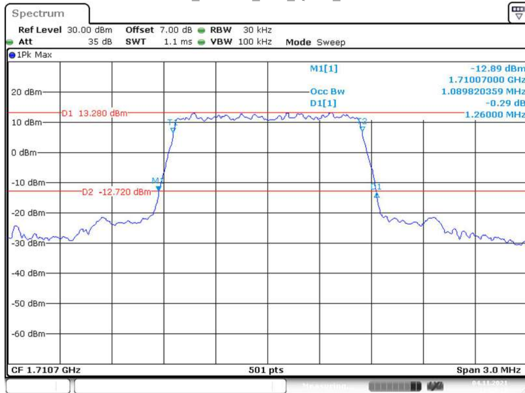
Band 4_1.4 MHz_Low_QPSK_RB6#0
