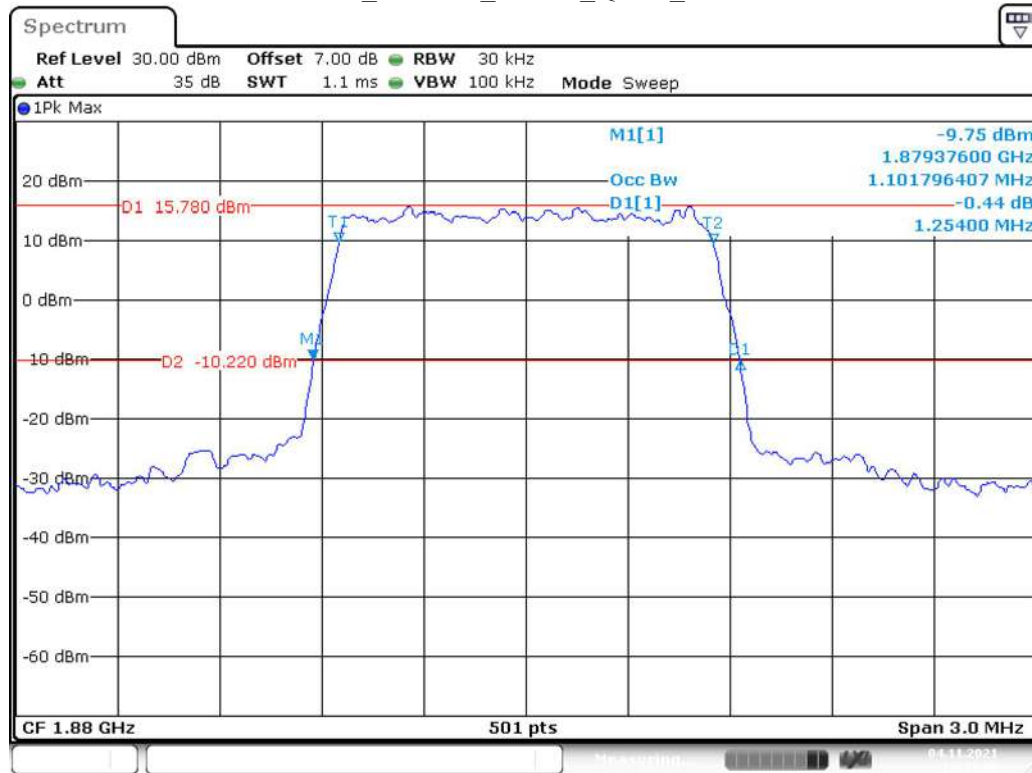
Band 2_1.4 MHz_Middle_QPSK_RB6#0
