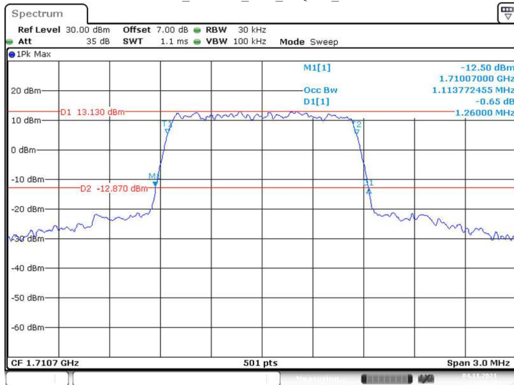
Band 4_1.4 MHz_Low_16QAM_RB6#0
