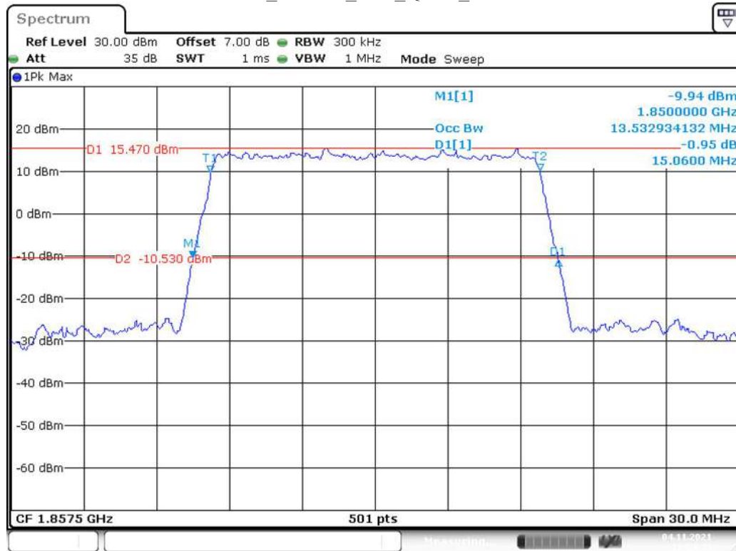
Band 2_15 MHz_Low_QPSK_RB75#0
