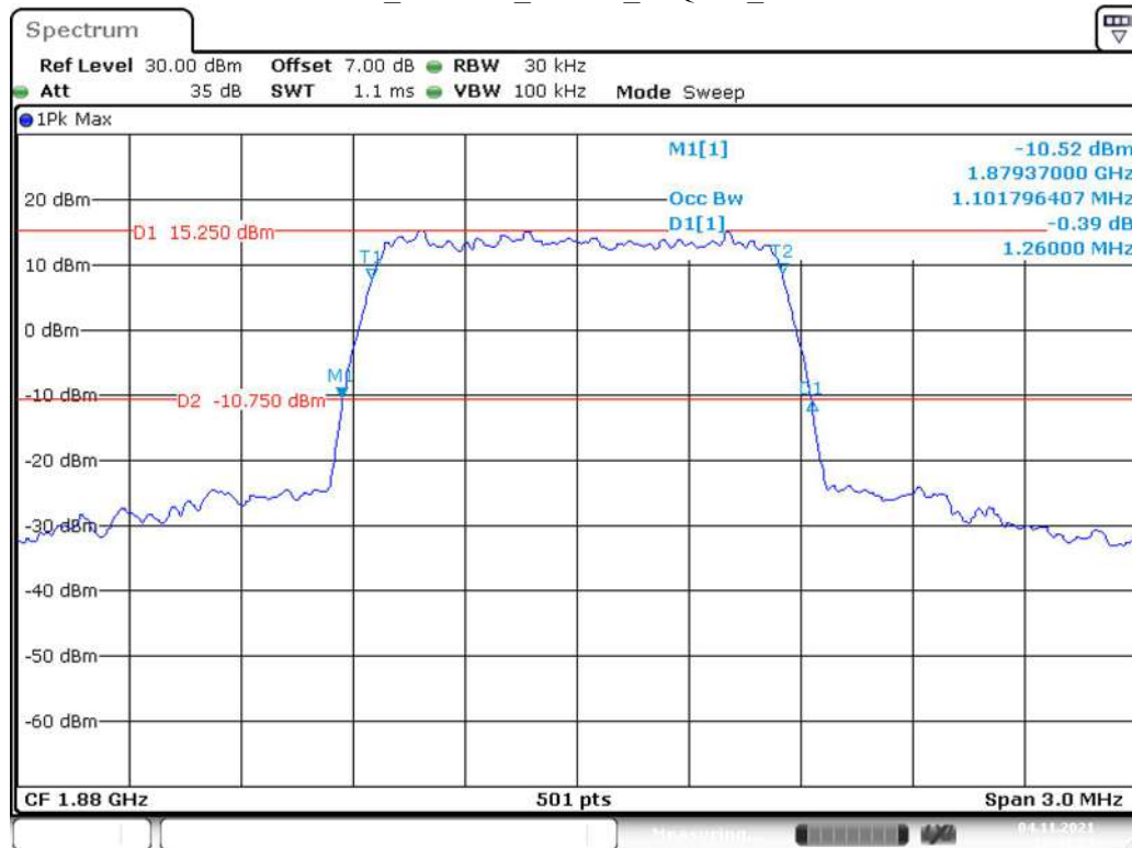
Band 2_1.4 MHz_Middle_16QAM_RB6#0
