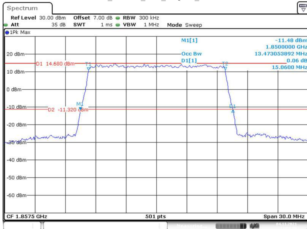
Band 2_15 MHz_Low_16QAM_RB75#0
