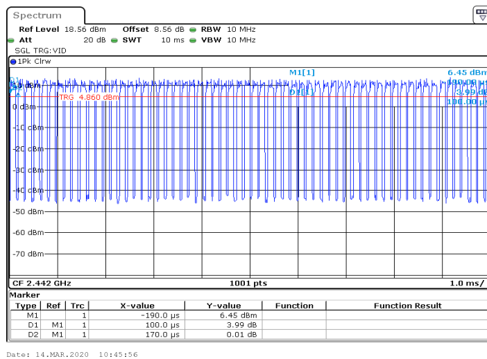
11N20SISO_Ant1_2442
