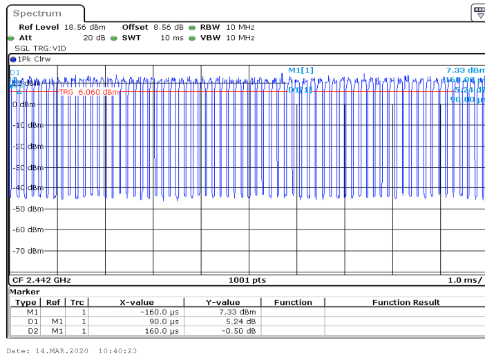
11N20SISO_Ant1_2442
