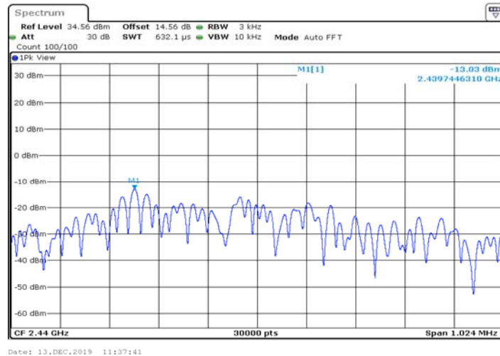
BLE_BT4.0_Ant1_2440
