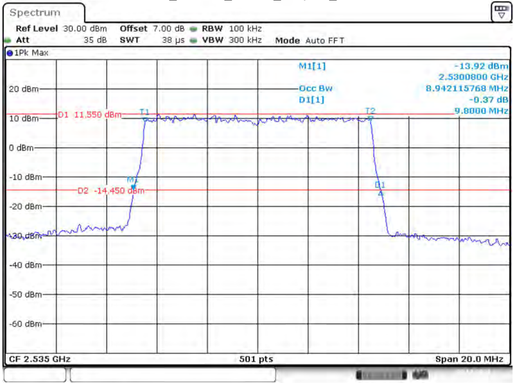
Band 7_10 MHz_Middle_16QAM_RB50#0
