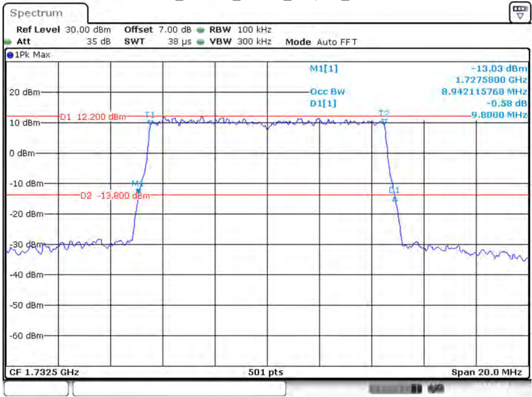
Band 4_10 MHz_Middle_16QAM_RB50#0
