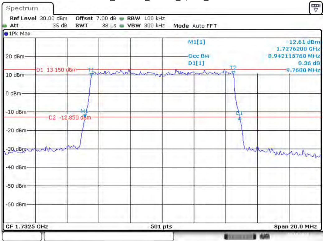
Band 4_10 MHz_Middle_QPSK_RB50#0
