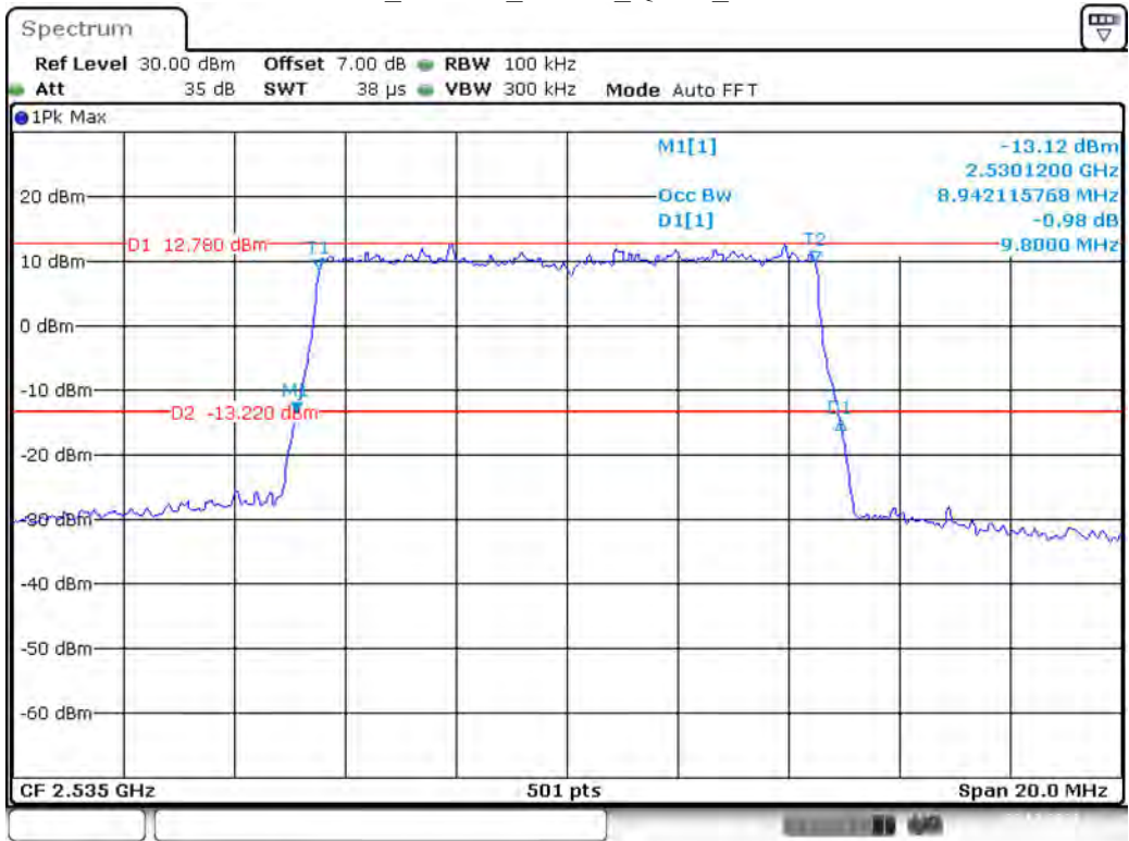
Band 7_10 MHz_Middle_QPSK_RB50#0
