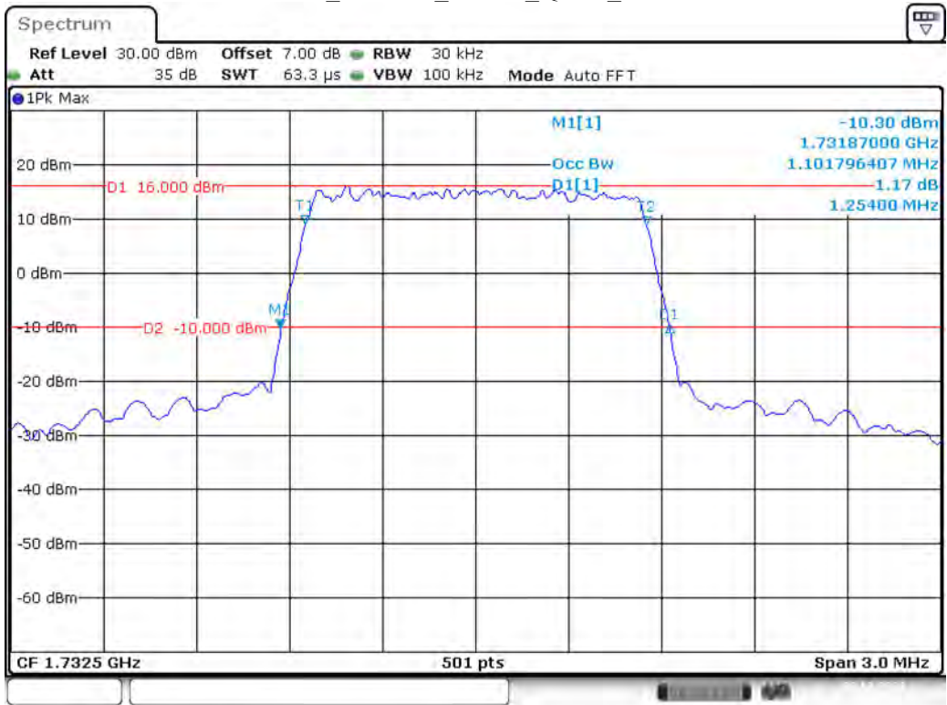
Band 4_1.4 MHz_Middle_QPSK_RB6#0
