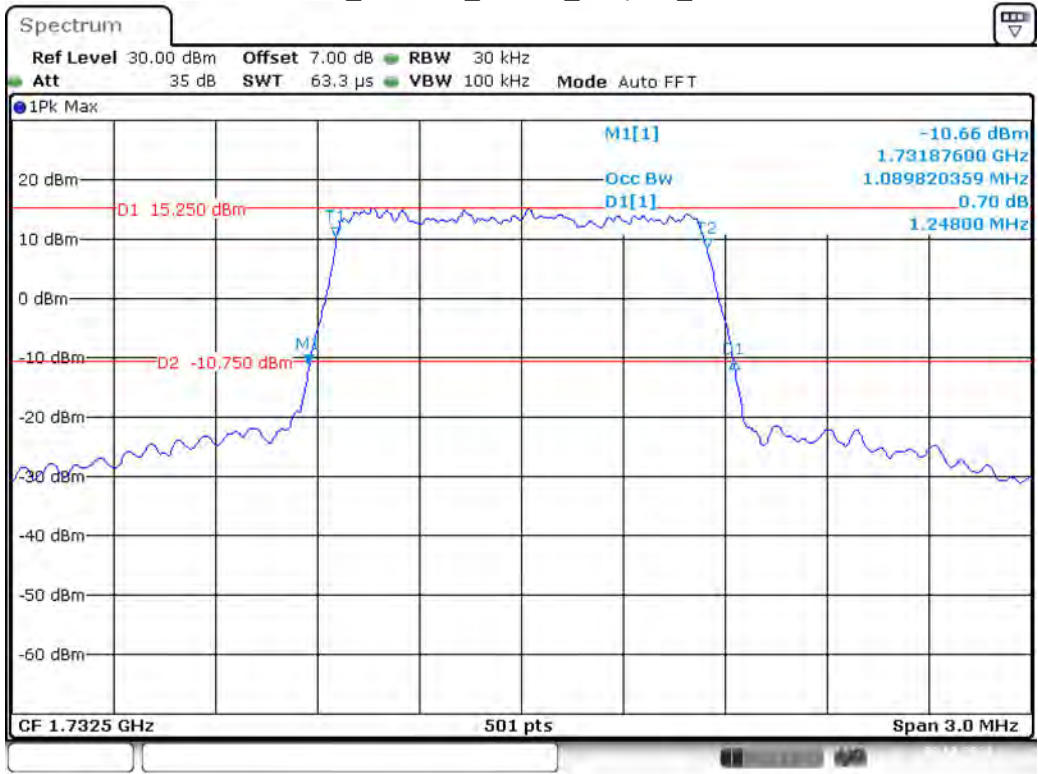
Band 4_1.4 MHz_Middle_16QAM_RB6#0
