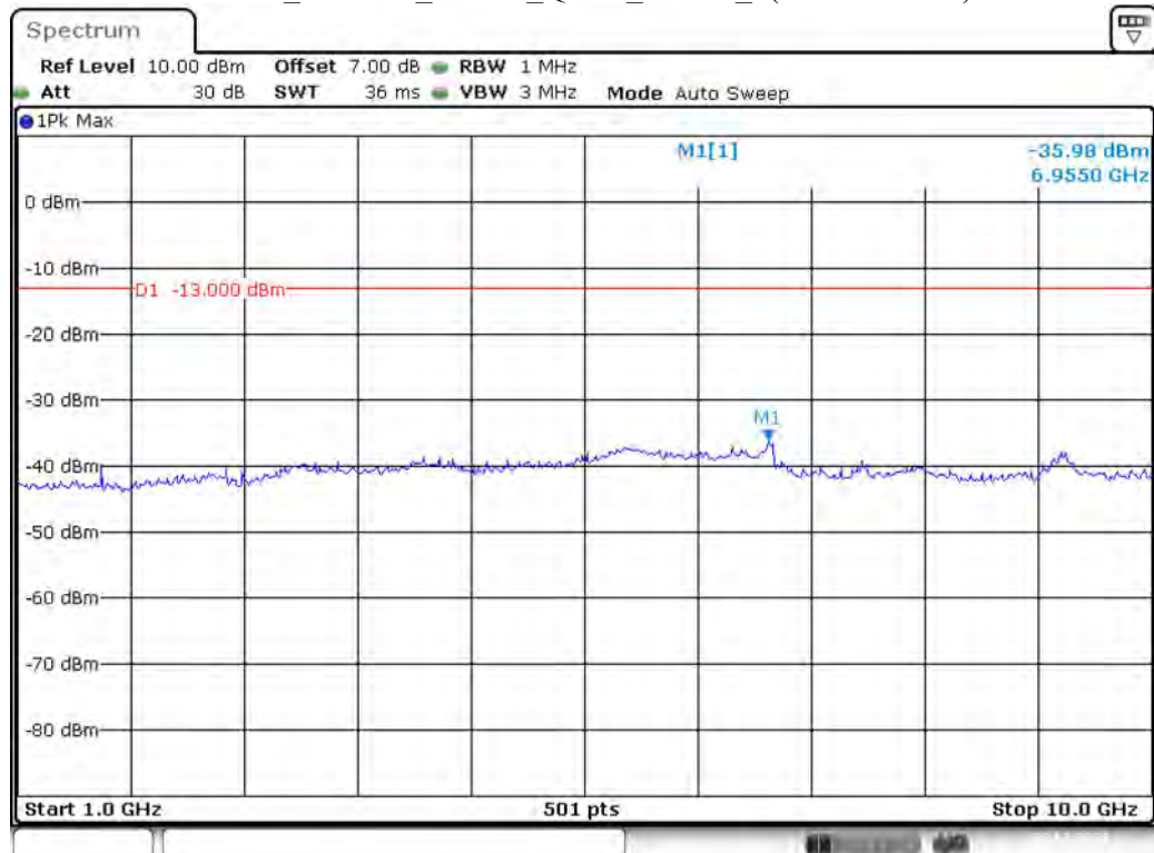
Band 5_1.4 MHz_Middle_QPSK_RB6#0_2(1GHz-10GHz)
