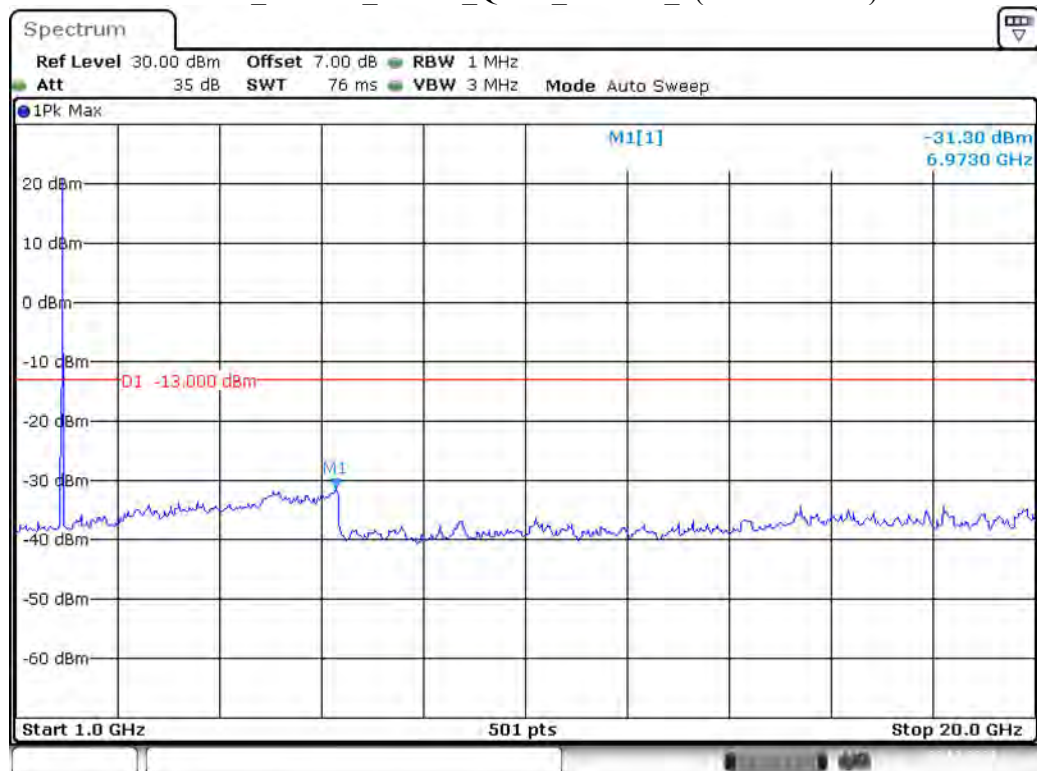
Band 2_10 MHz_Middle_QPSK_RB50#0_2(1GHz-20GHz)
