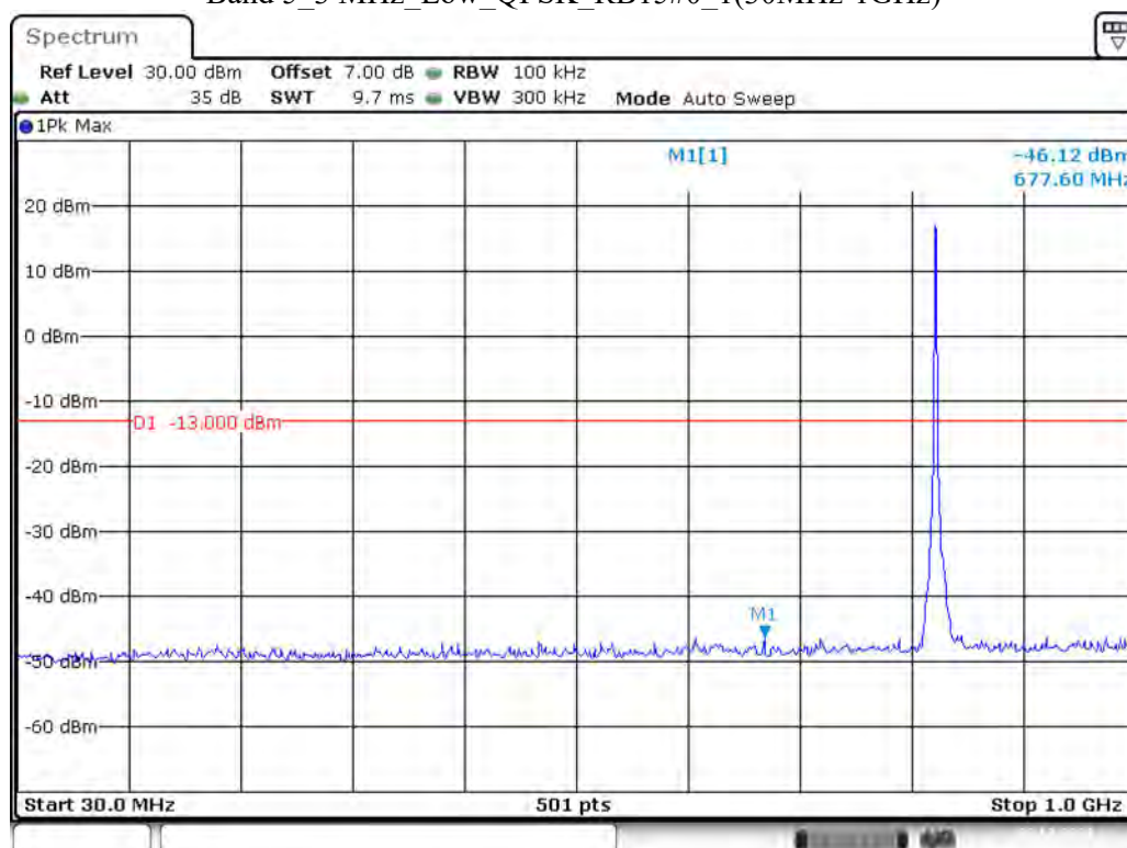
Band 5 3 MHz Low QPSK RB15#0 1(30MHz-1GHz)
