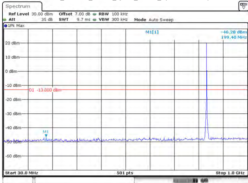
Band 5_1.4 MHz_Middle_QPSK_RB6#0_1(30MHz-1GHz)
