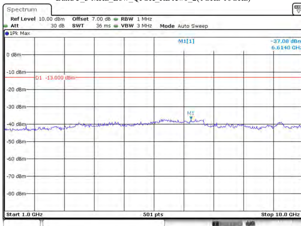
Band 5 3 MHz Low QPSK RB15#0 2(1GHz-10GHz)
