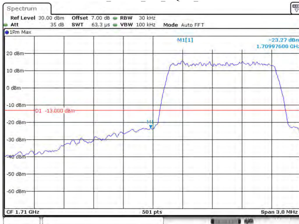
Band 4_1.4 MHz_Low_16QAM_RB6#0
