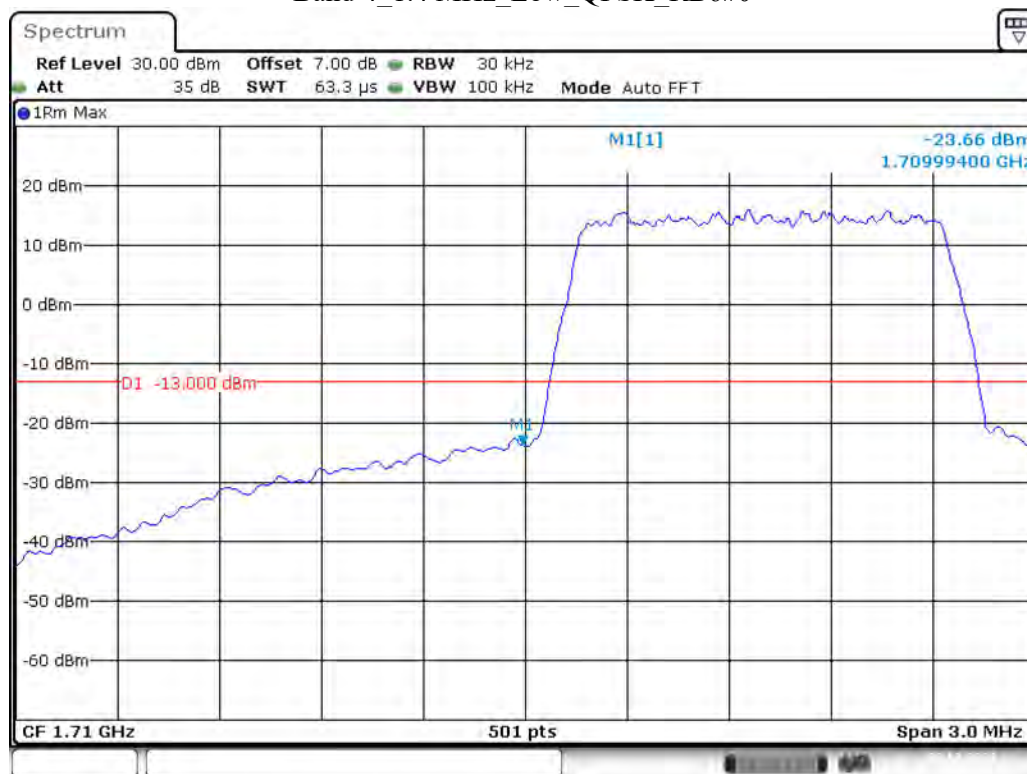
Band 4_1.4 MHz_Low_QPSK_RB6#0
