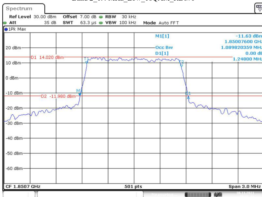
Band 2_1.4 MHz_Low_16QAM_RB6#0
