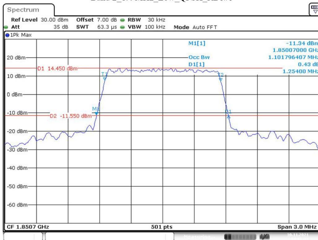
Band 2_1.4 MHz_Low_QPSK_RB6#0
