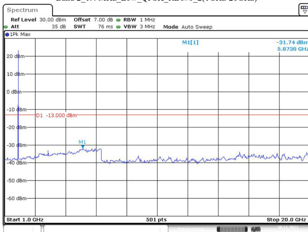
Band 2_1.4 MHz_Low_QPSK_RB6#0_2(1GHz-20GHz)
