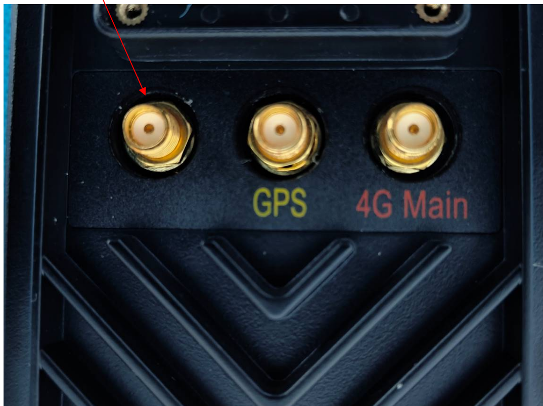
LTE DIV Antenna port(only RX)
