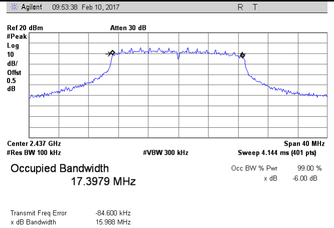
802.11n20 6dB Bandwidth - Mid CH 2437
