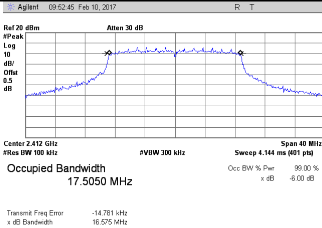
802.11n20 6dB Bandwidth - Low CH 2412
