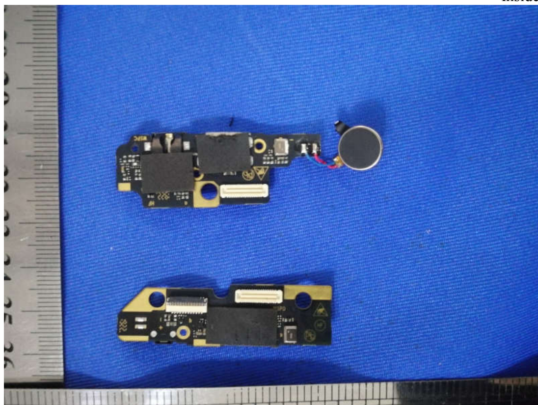
Figure 21 Inside of the EUT
