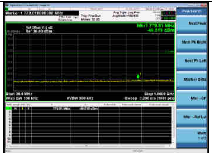
Test Mode: IEEE 802.11n HT20 Test CH1: 2412MHz
