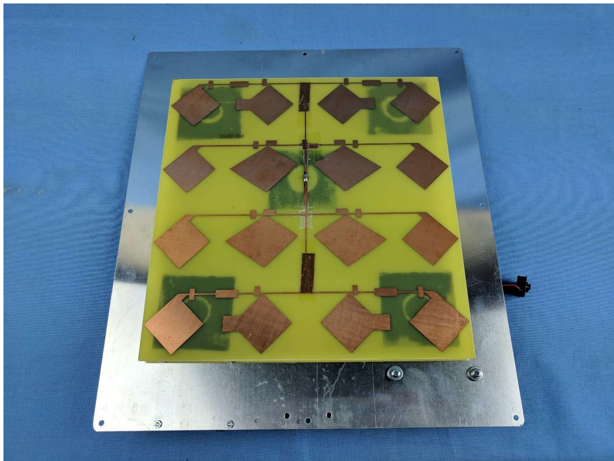
DV11AC Antenna
