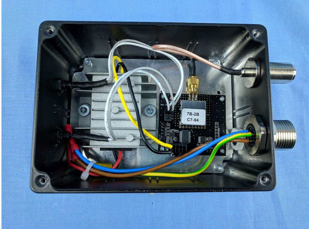
DV31DC Internal
