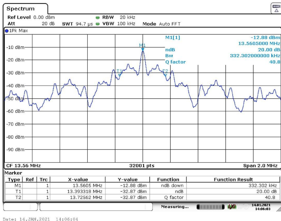
Figure 6: 20 dB bandwidth
