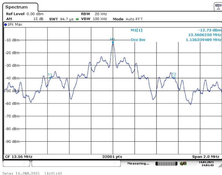
Figure 7: 99% occupied bandwidth
