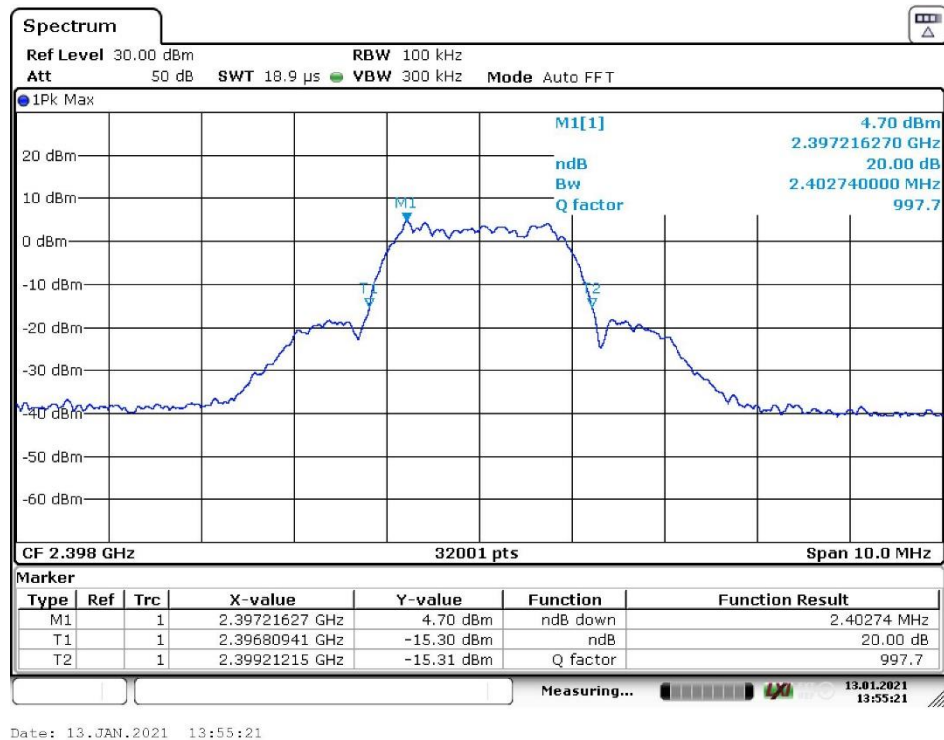
Figure 6: Emission Bandwidth, HIGH channel (bottom antenna)
