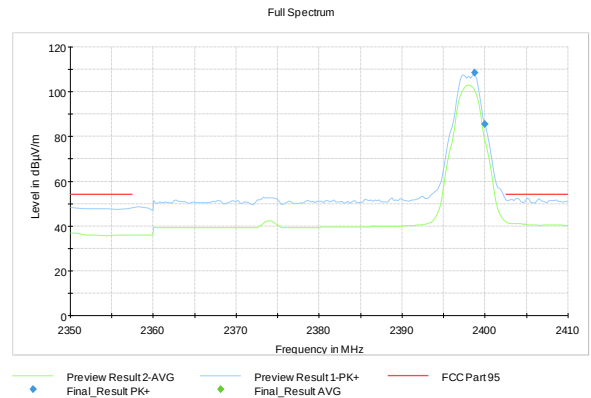
Figure 32: Upper band-edge (top antenna)
