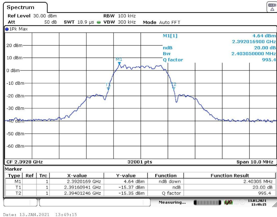
Figure 5: Emission Bandwidth, LOW channel (bottom antenna)
