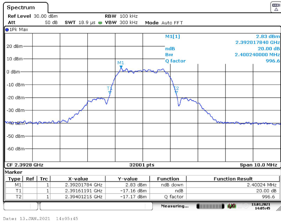
Figure 7: Emission Bandwidth, LOW channel (top antenna)
