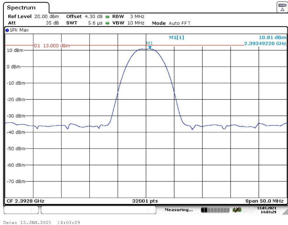
Figure 3: Radiated Power, LOW channel (top antenna)
