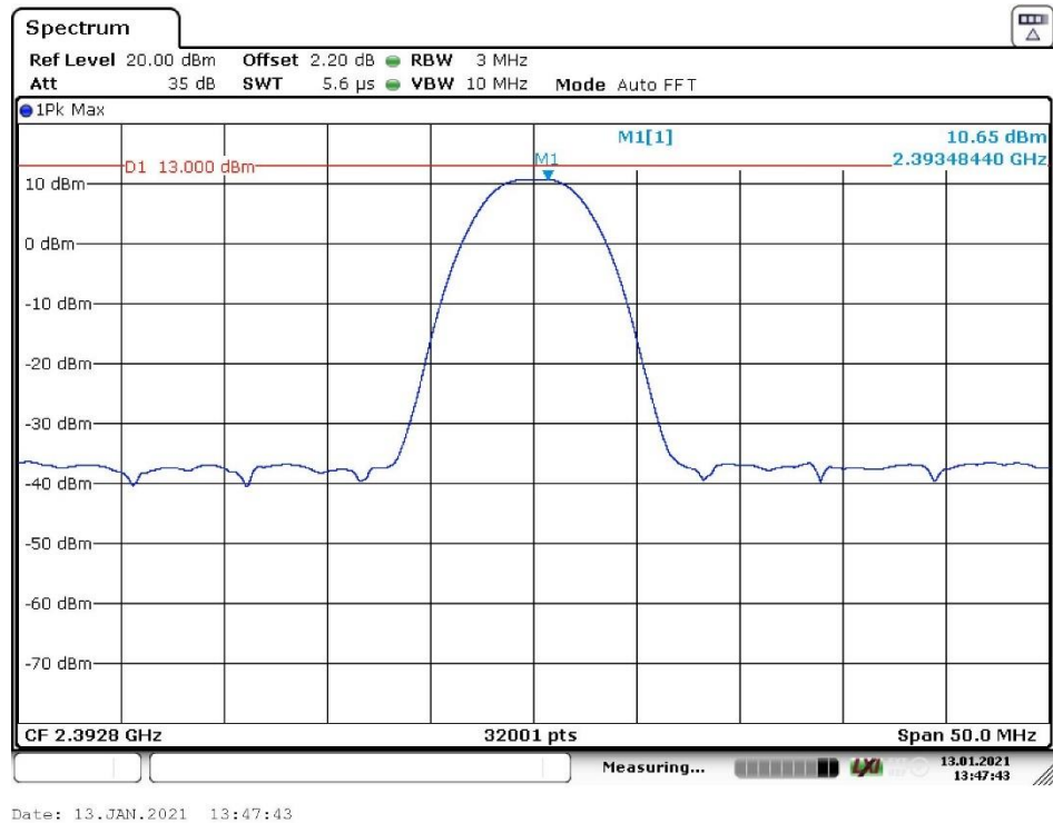
Figure 1: Radiated Power, LOW channel (bottom antenna)
