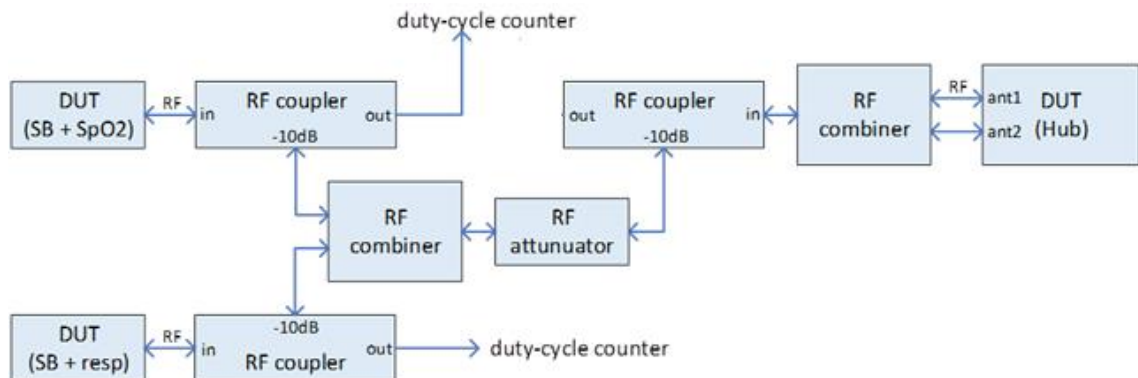
Figure 2: Duty cycle measurement setup
