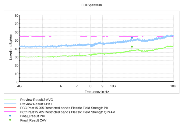
Figure 12: LOW channel (4 GHz – 18 GHz)
