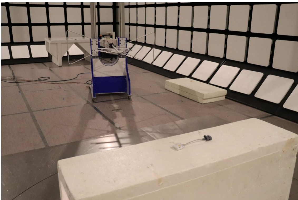
Photograph 2. Test Setup for Radiated Emissions 30 – 1000 MHz
