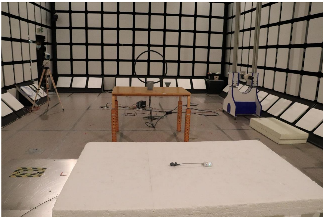
Photograph 1. Test Setup for Radiated Emissions 9 kHz – 30 MHz
