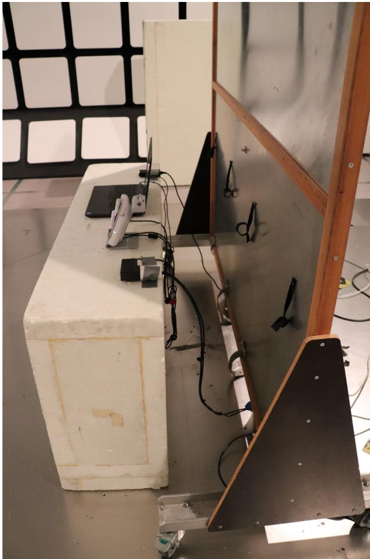
Photograph 5. Test Setup for Conducted Emissions 150 kHz – 30 MHz
