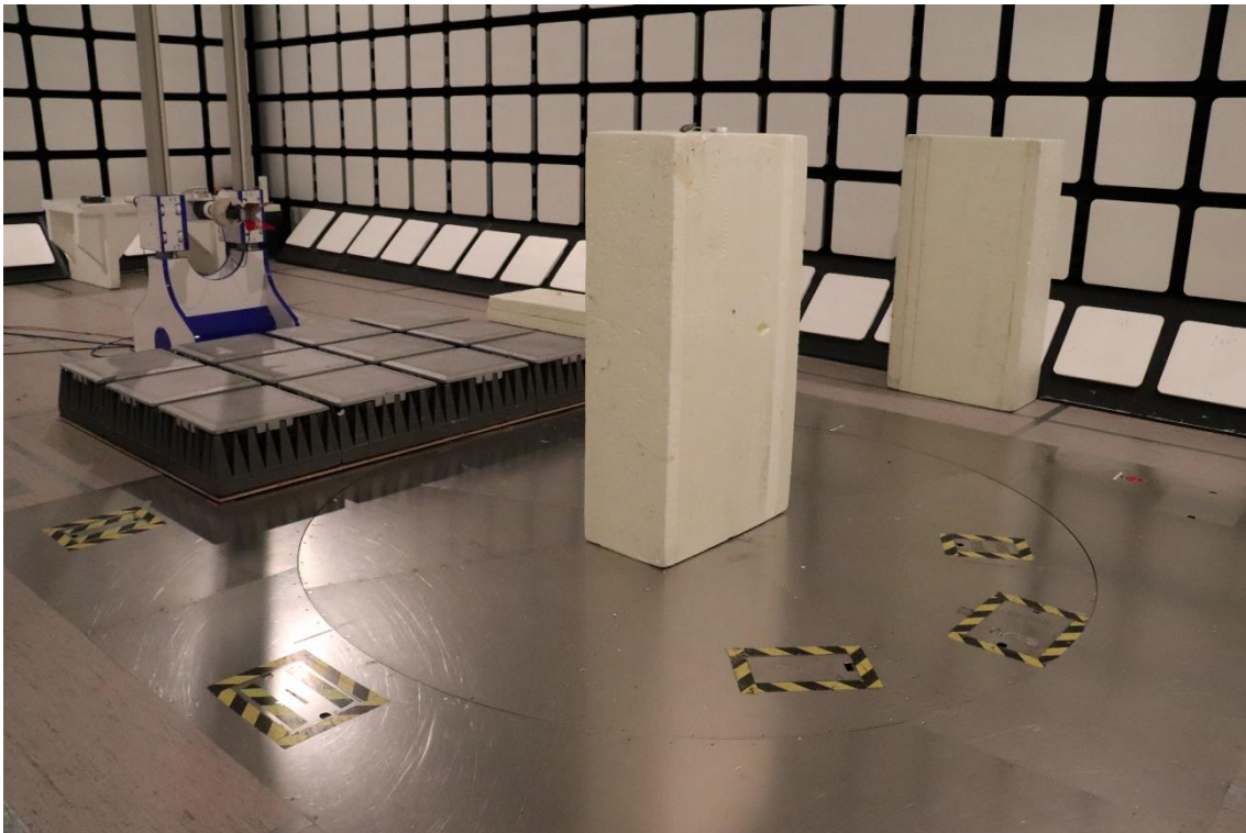
Photograph 3. Test Setup for Radiated Emissions 1 – 18 GHz
