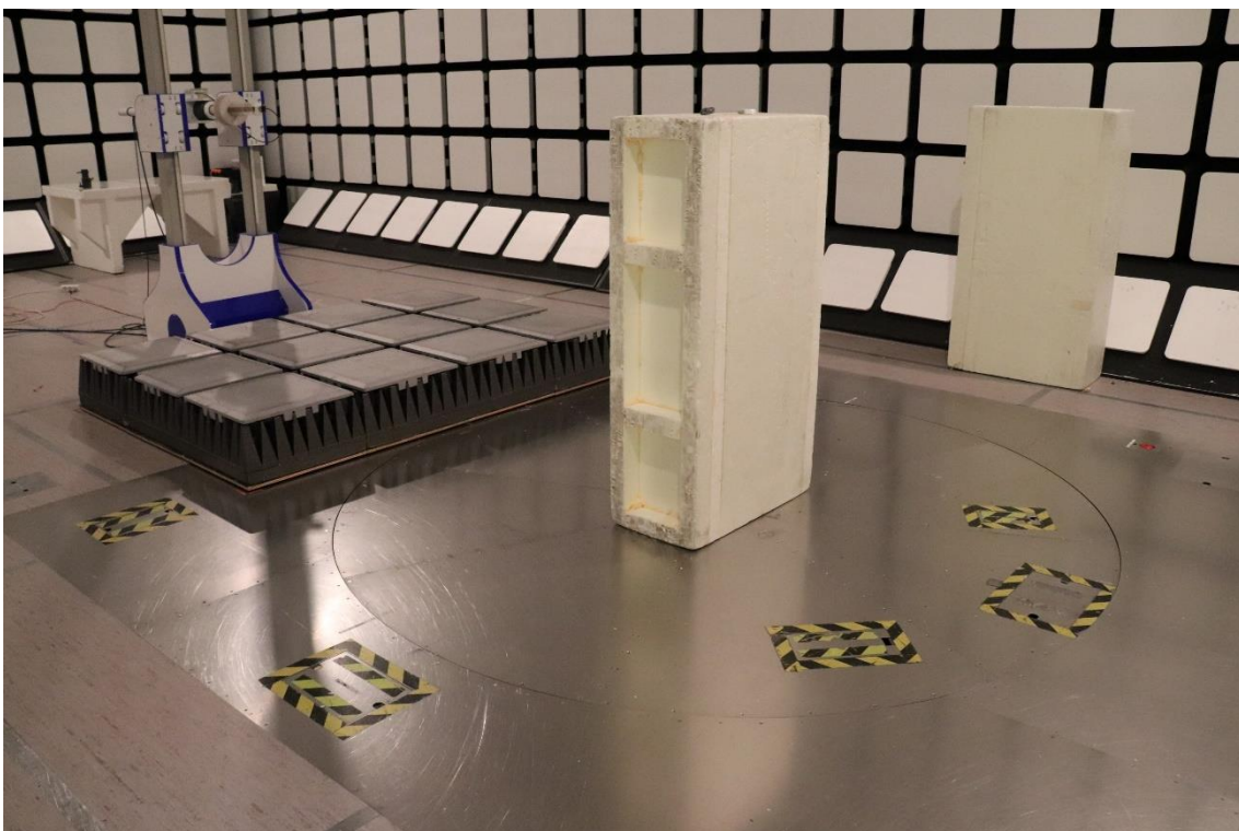
Photograph 4. Test Setup for Radiated Emissions 18 – 26.5 GHz
