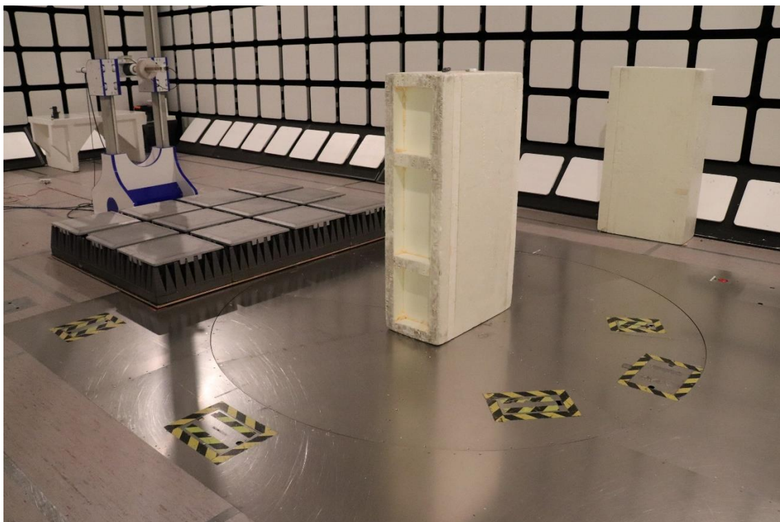
Photograph 4. Test Setup for Radiated Emissions 18 – 24 GHz
